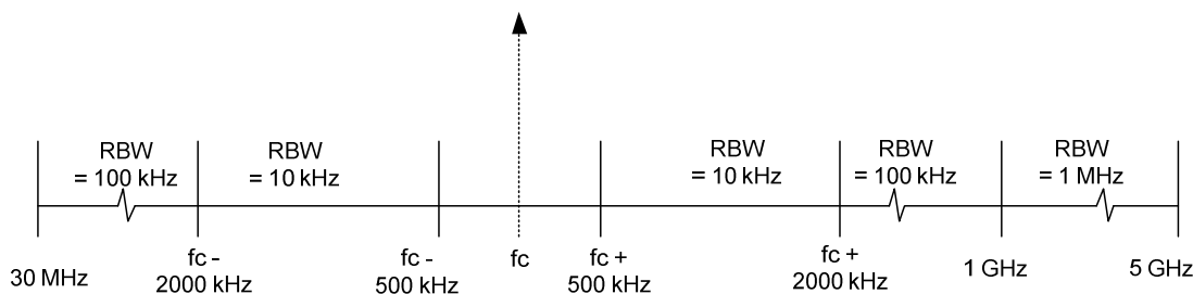
Figure 4: Resolution bandwidths for spurious emissions
