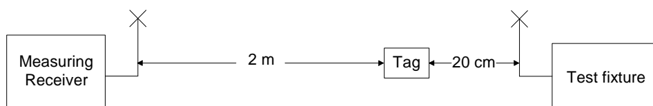
Figure 6: Measurement of tag emissions
