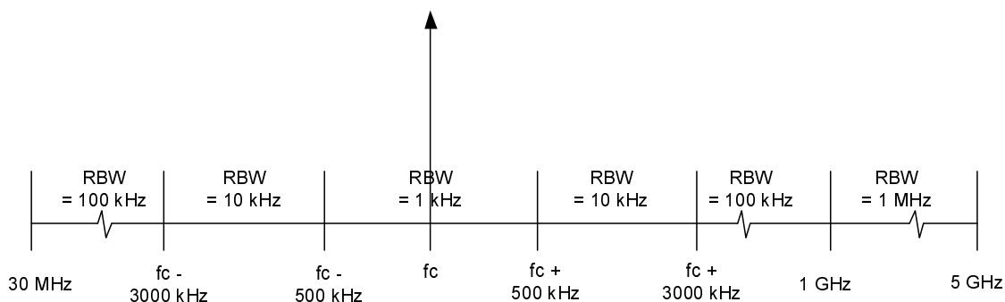
Figure 7: Resolution bandwidths for tag emissions
