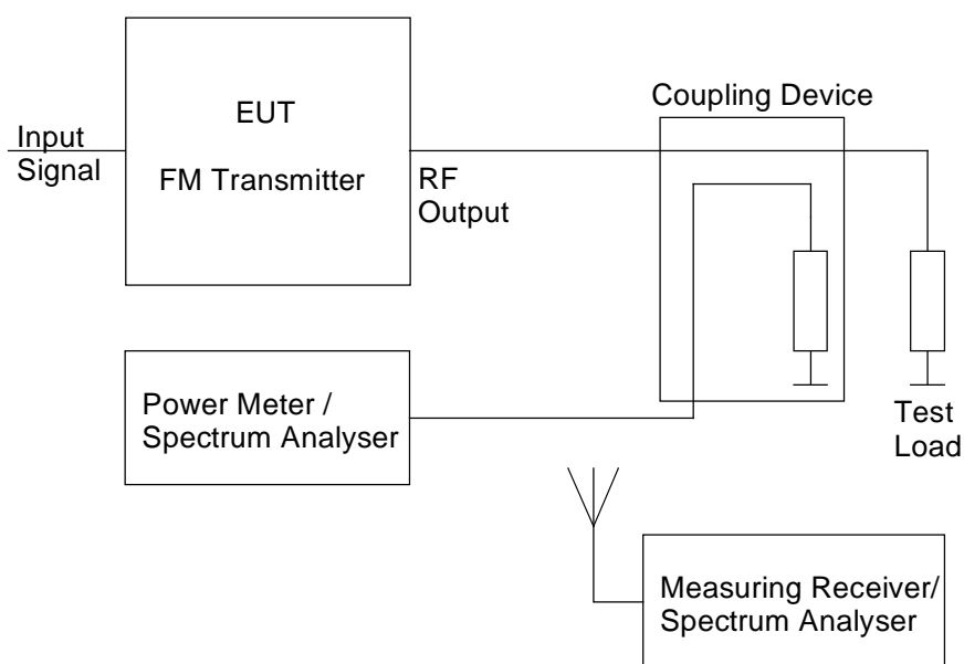
Figure B.5: Testing arrangement for cabinet radiation
