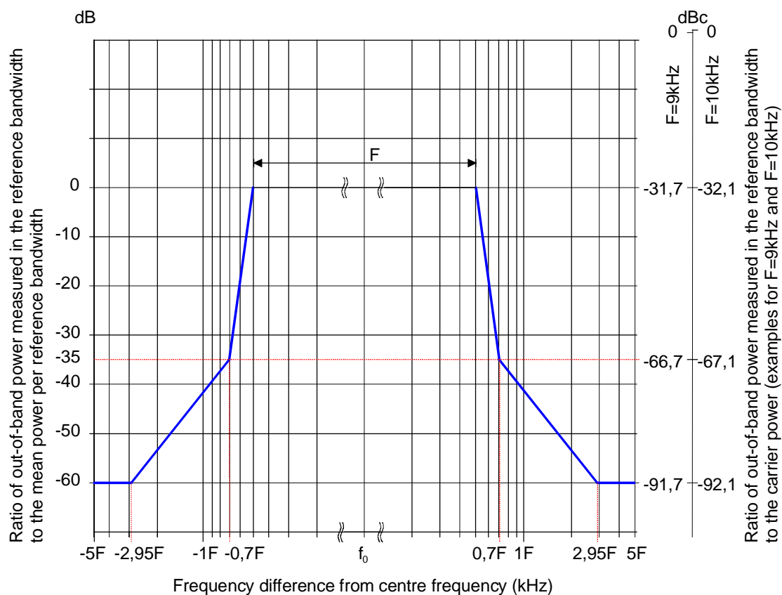
Figure 4.2: Out of band emission limits shown on a logarithmic axis
