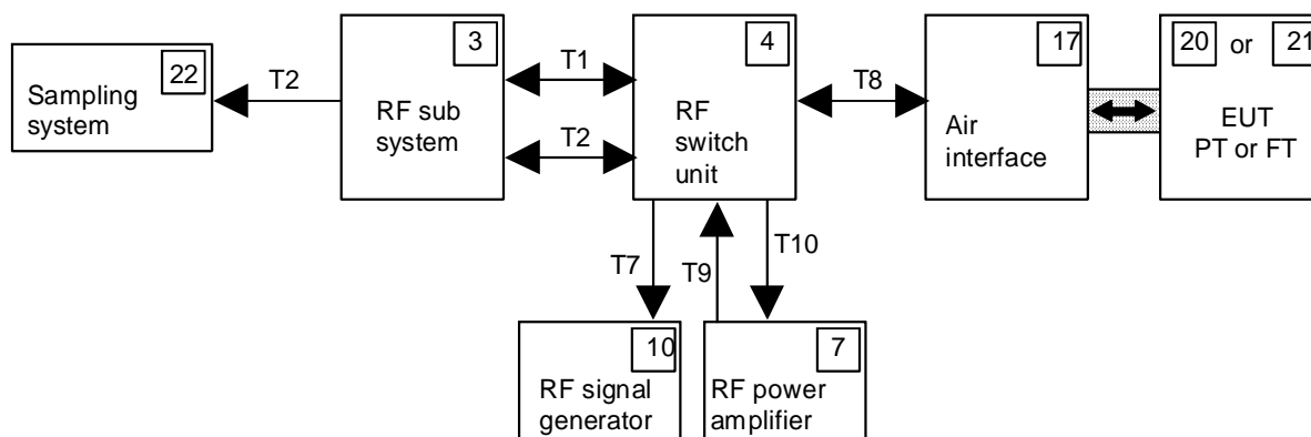
Figure 23: Test setup 5
