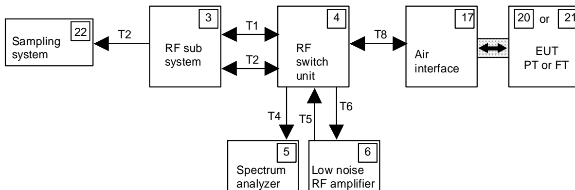
Figure 22: Test setup 4
