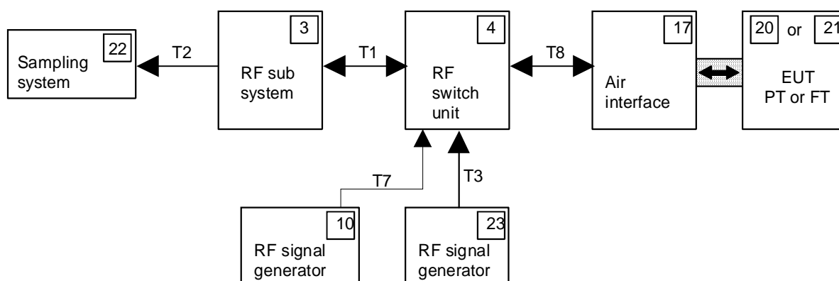
Figure 21: Test setup 3
