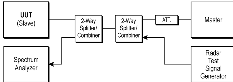
Figure 5: Set-up C
