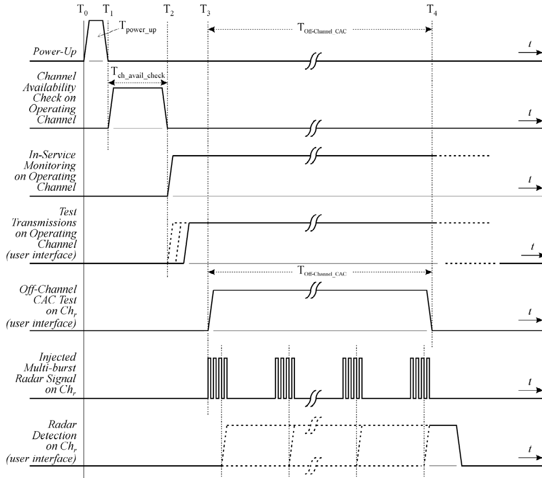
Figure 9: Example of timing for radar testing during the Off-Channel CAC
