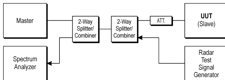
Figure 4: Set-up B
