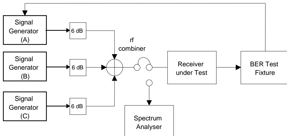
Figure 17: Intermodulation measurement
