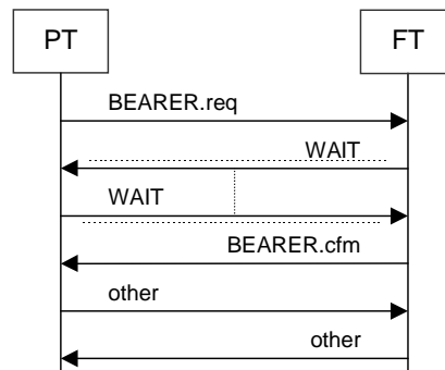
Figure 10: PT initiated setup of additional duplex bearer
