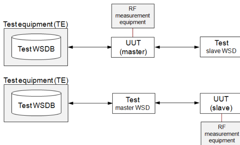
Figure 2: Test set-up
