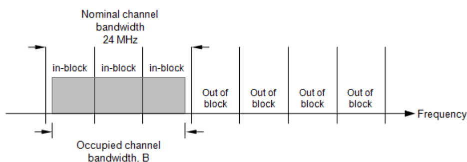
Figure E.3: Group of contiguous DTT channels
