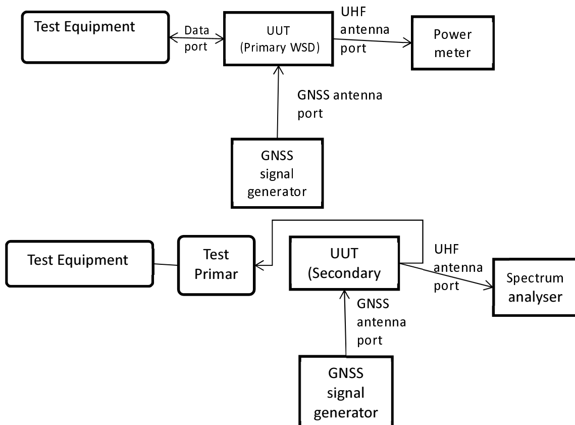
Figure 8: Test arrangement for Geo-location capability
