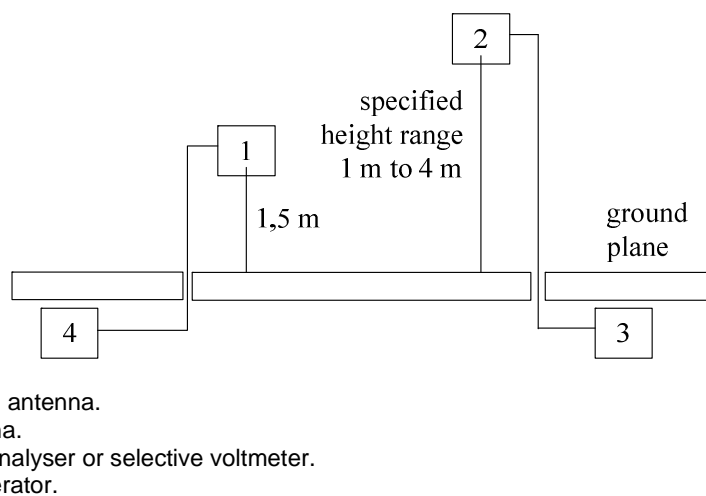
Figure C.2: Measurement arrangement 2
