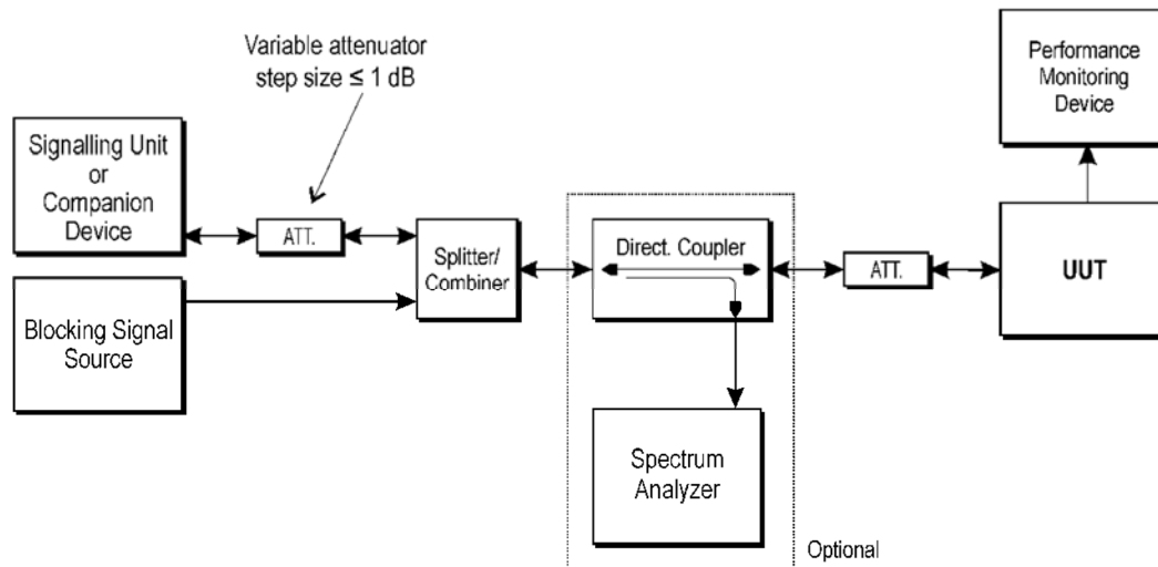
Figure 4: Test Set-up for receiver blocking
