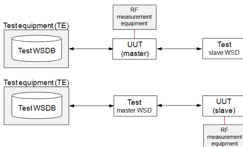
Figure 2: Test set-up
