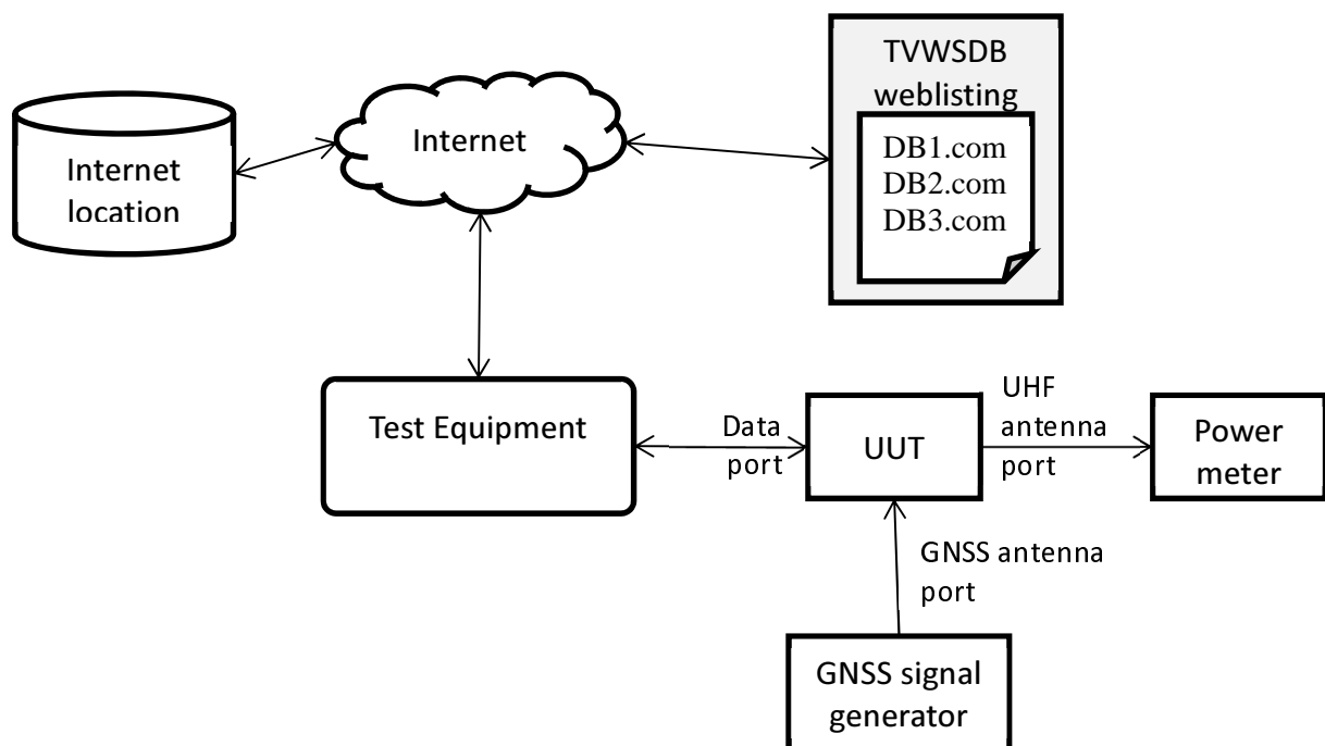
Figure 4a: Test arrangement for test database identification and access
