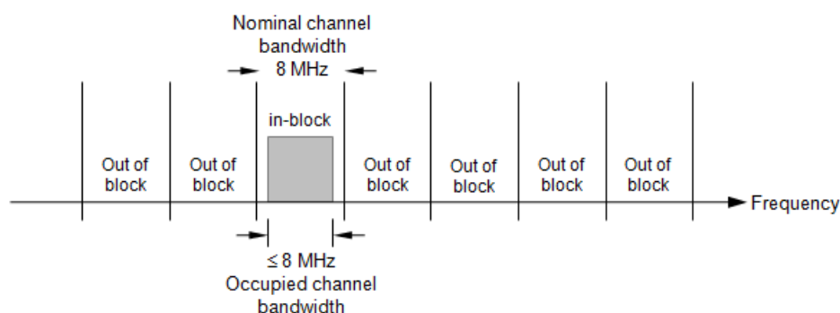
Figure E.2: Single DTT channel
