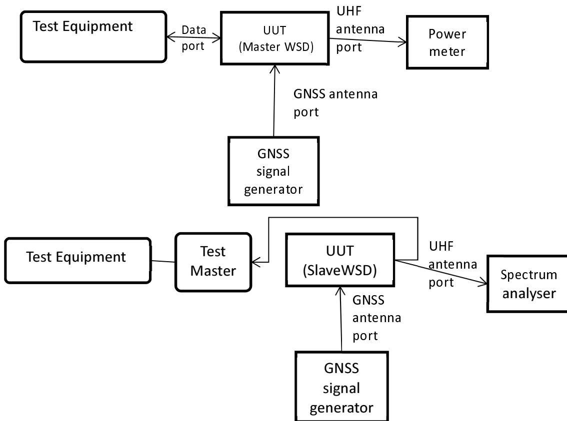
Figure 5: Test arrangement for Geo-location capability
