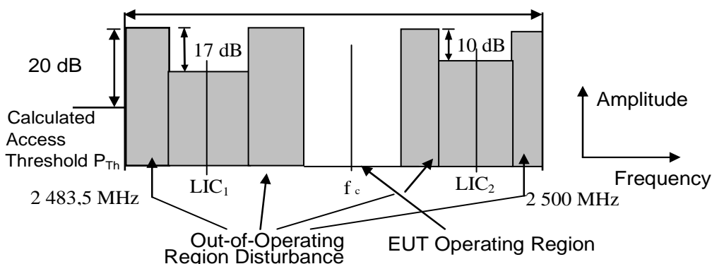
Figure 4: Spectrum Mask for Test
