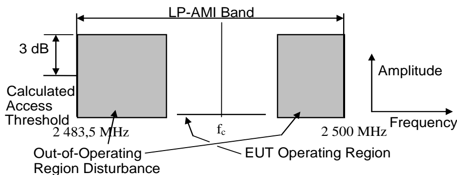
Figure 2: Spectrum Mask for Test of clauses 5.3.3.3.1 and 5.3.3.3.2
