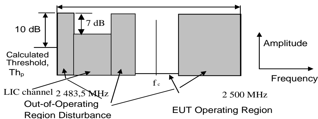
Figure 3: Spectrum Mask for Test
