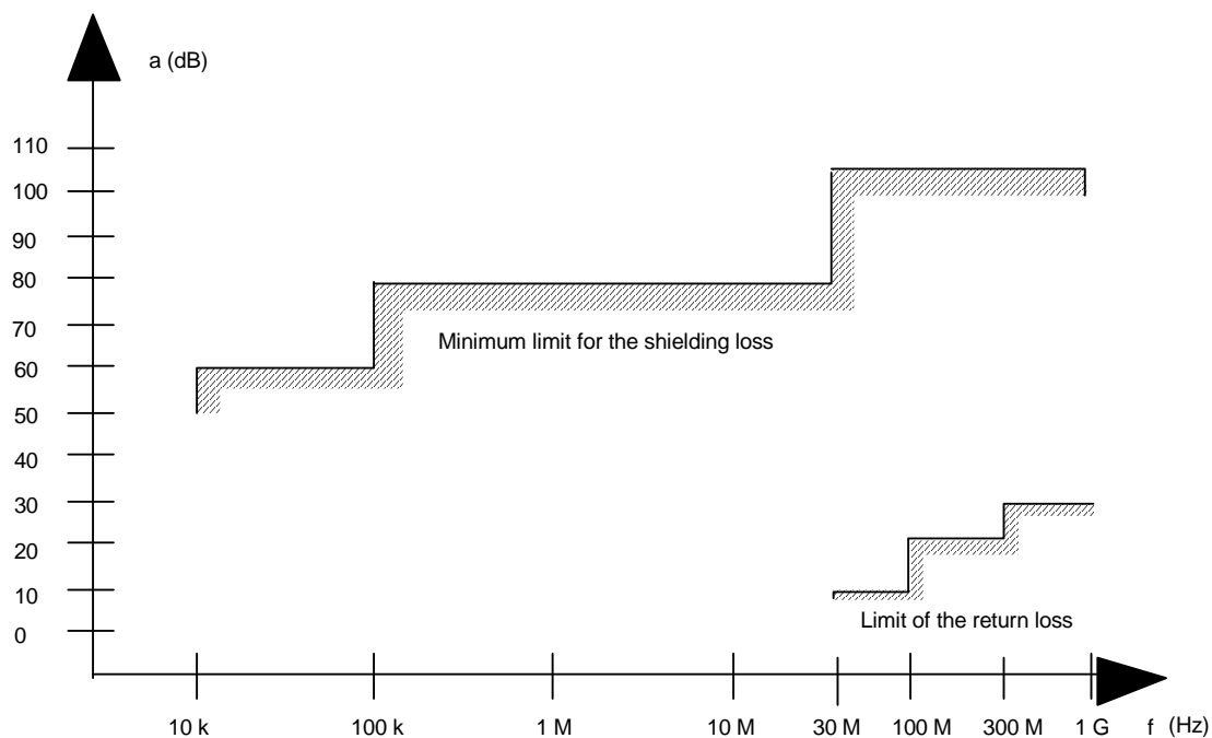
Figure B.5: Specification for shielding and reflections
