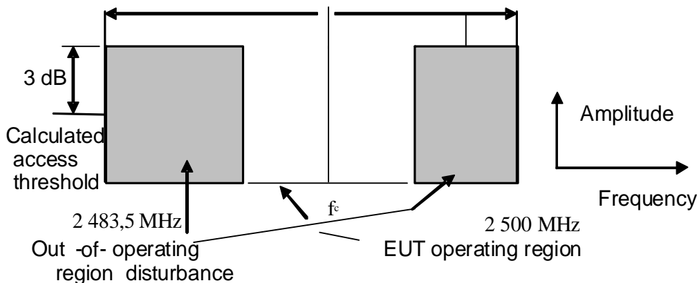
Figure 1: Spectrum Mask for Test of clauses 5.3.3.2.1, 5.3.3.2.2 and 5.3.3.2.3
