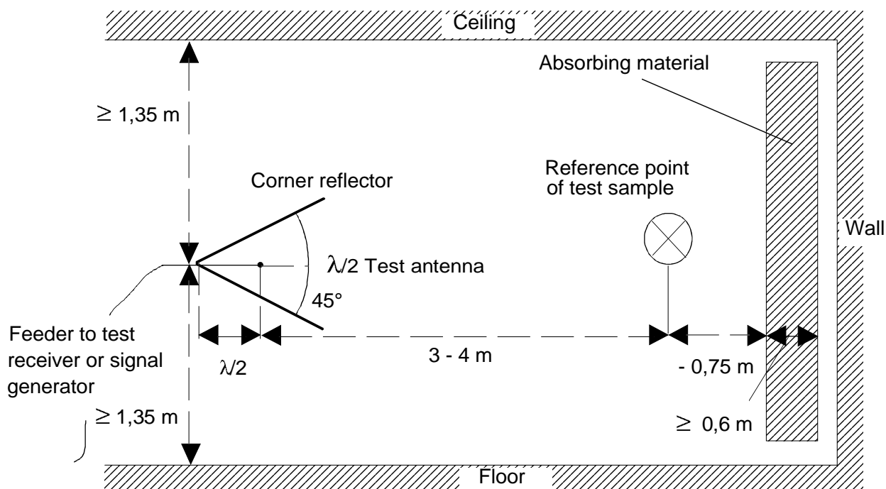
Figure B.4: Indoors site arrangement (shown for horizontal polarization)
