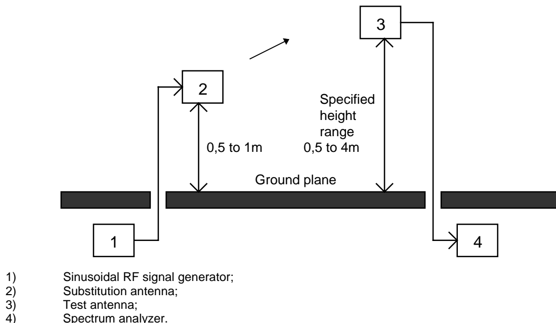
Figure 4: Measurement arrangement No. 2
