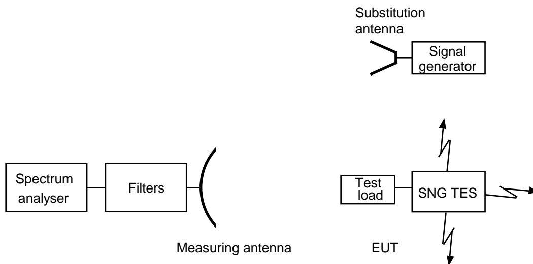
Figure 5: Test arrangement - Spurious radiation measurement above 1,0 GHz
