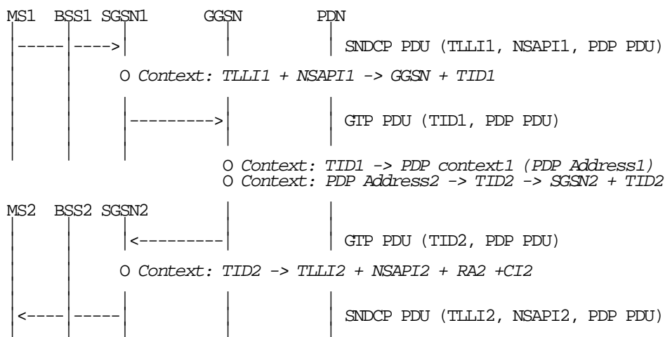
Figure C.3: MS-to-MS Data Routeing via the Same GGSN
