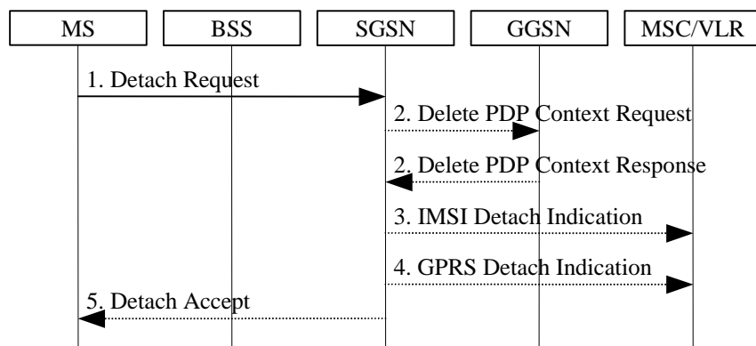
Figure 19: MS-Initiated Combined GPRS / IMSI Detach Procedure
