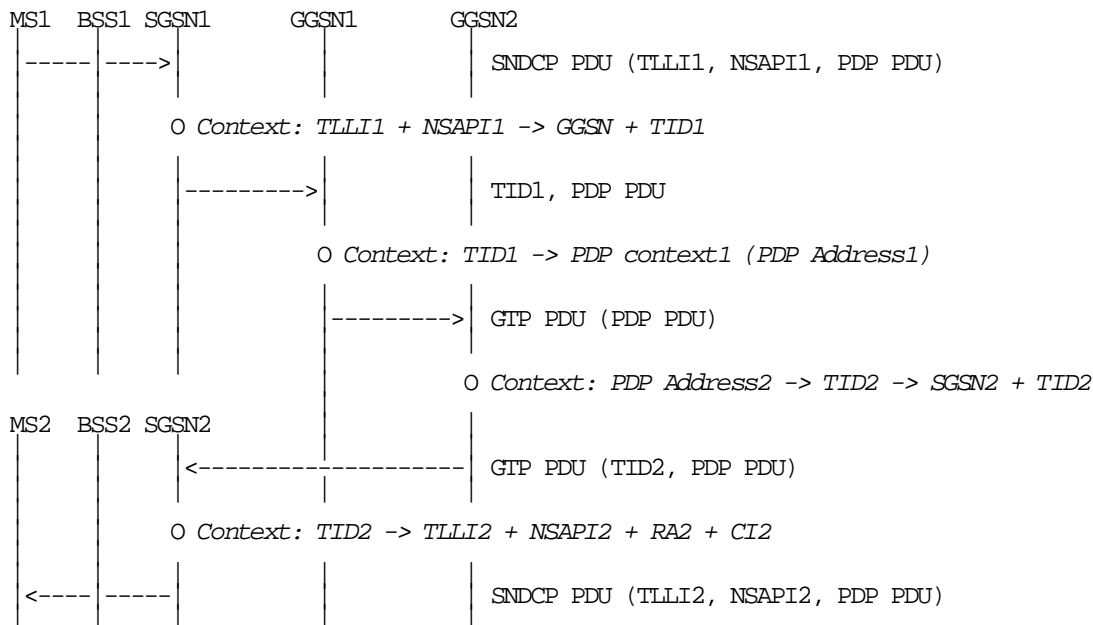
Figure C.4: MS-to-MS Data Routeing via Different GGSNs
