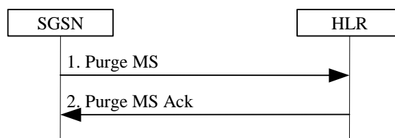
Figure 22: Purge Procedure
