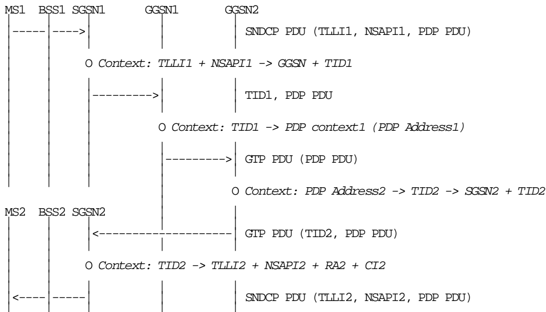
Figure B.4: MS-to-MS Data Routeing via Different GGSNs
