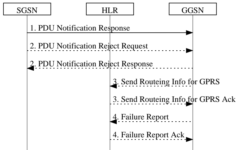
Figure 37: Protection Procedure
