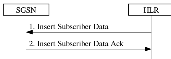
Figure 31: Insert Subscriber Data Procedure
