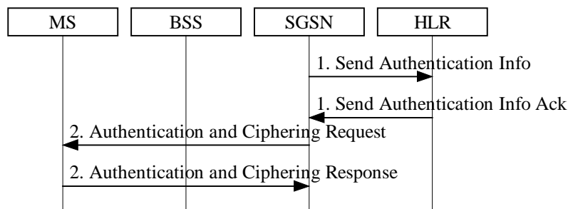
Figure 23: Authentication Procedure
