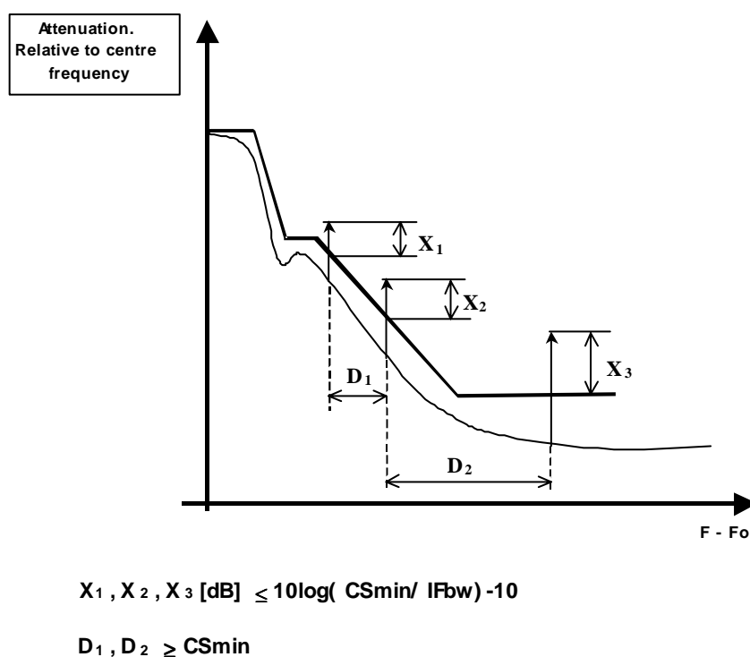
Figure 2C: CW lines exceeding the spectrum mask (typical example)
