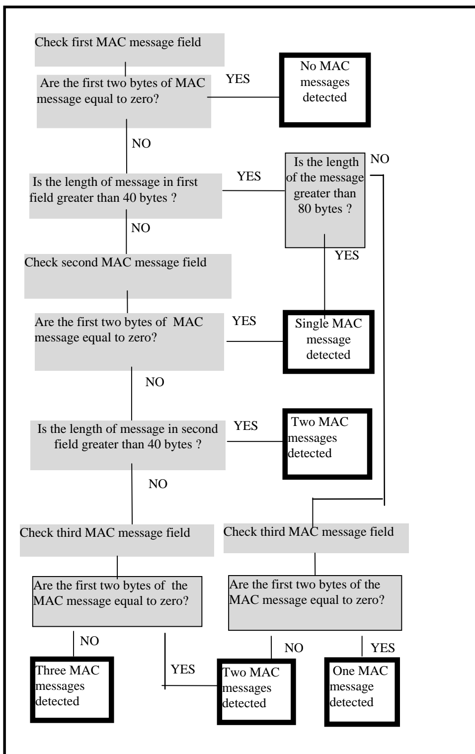
Figure 25: Algorithm when MAC message are sent IB downstream
