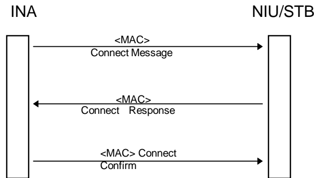
Figure 30: Connection signalling
