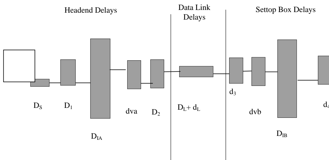
Figure 22. System model for timing analysis
