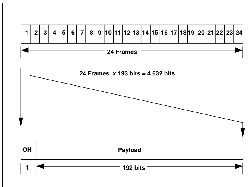
Figure 15: SL-ESF frame structure
