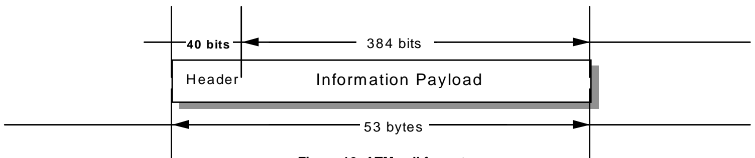
Figure 16: ATM cell format
