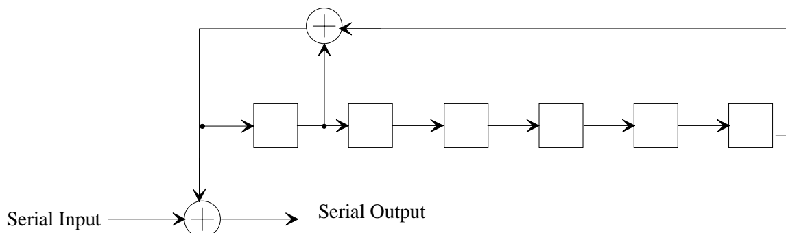
Figure 13: Randomizer
