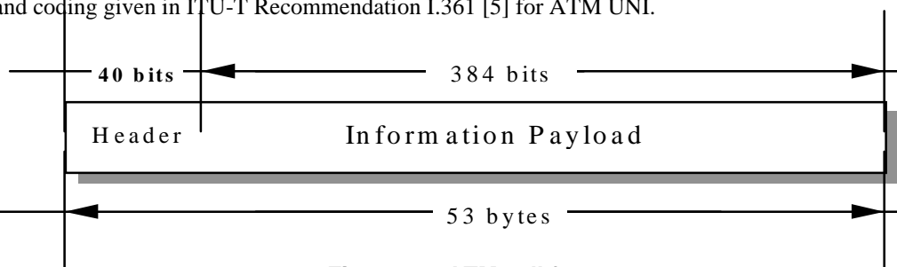
Figure 20: ATM cell format
