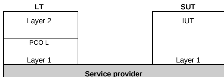
Figure 1: Remote test method
