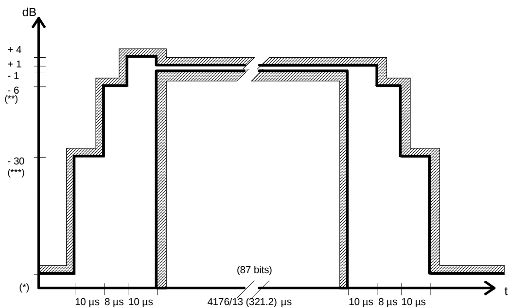
Time mask for access burst (AB)
