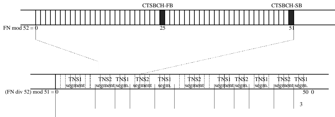
Figure 1 (clause 6.3.3): Structure of timeslot shifting sequence
