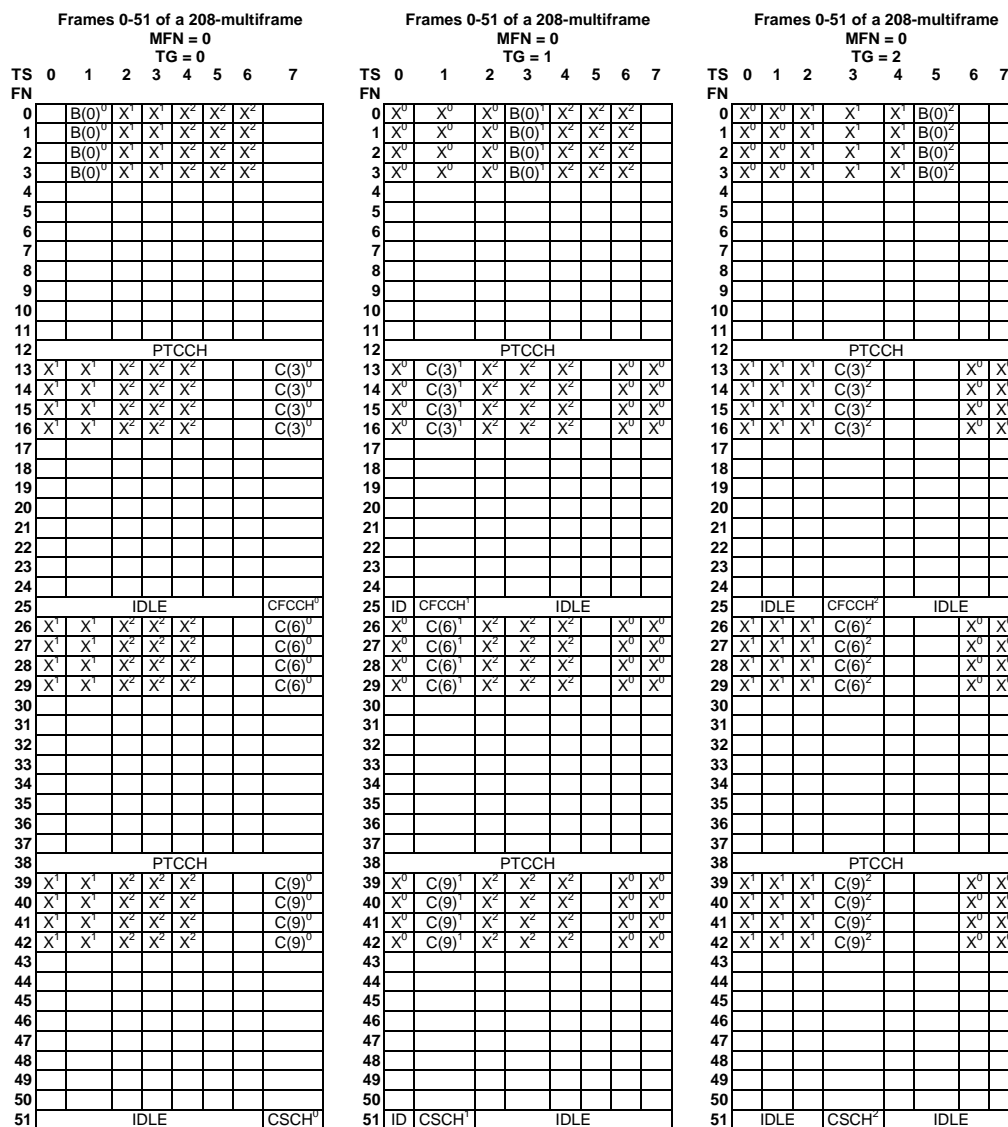
Figure D.4: COMPACT downlink 52-multiframe structure using 3 time groups for large cells (based on an assignment of 1 CPBCH and 3 CPCCCHs with NIB_CCCH_0 = NIB_CCCH_1 = NIB_CCCH_2 = 4, NIB_CPBCH_3 = 0). NIB_CCCH is not broadcast for serving cell time group
