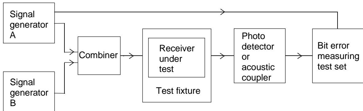
Figure 8: Measurement arrangement - adjacent channel selectivity
