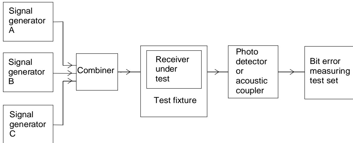
Figure 10: Measurement arrangement - intermodulation response rejection
