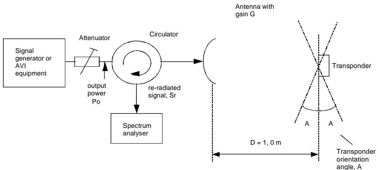
Figure 11: Measurement arrangement - transponder sensitivity
