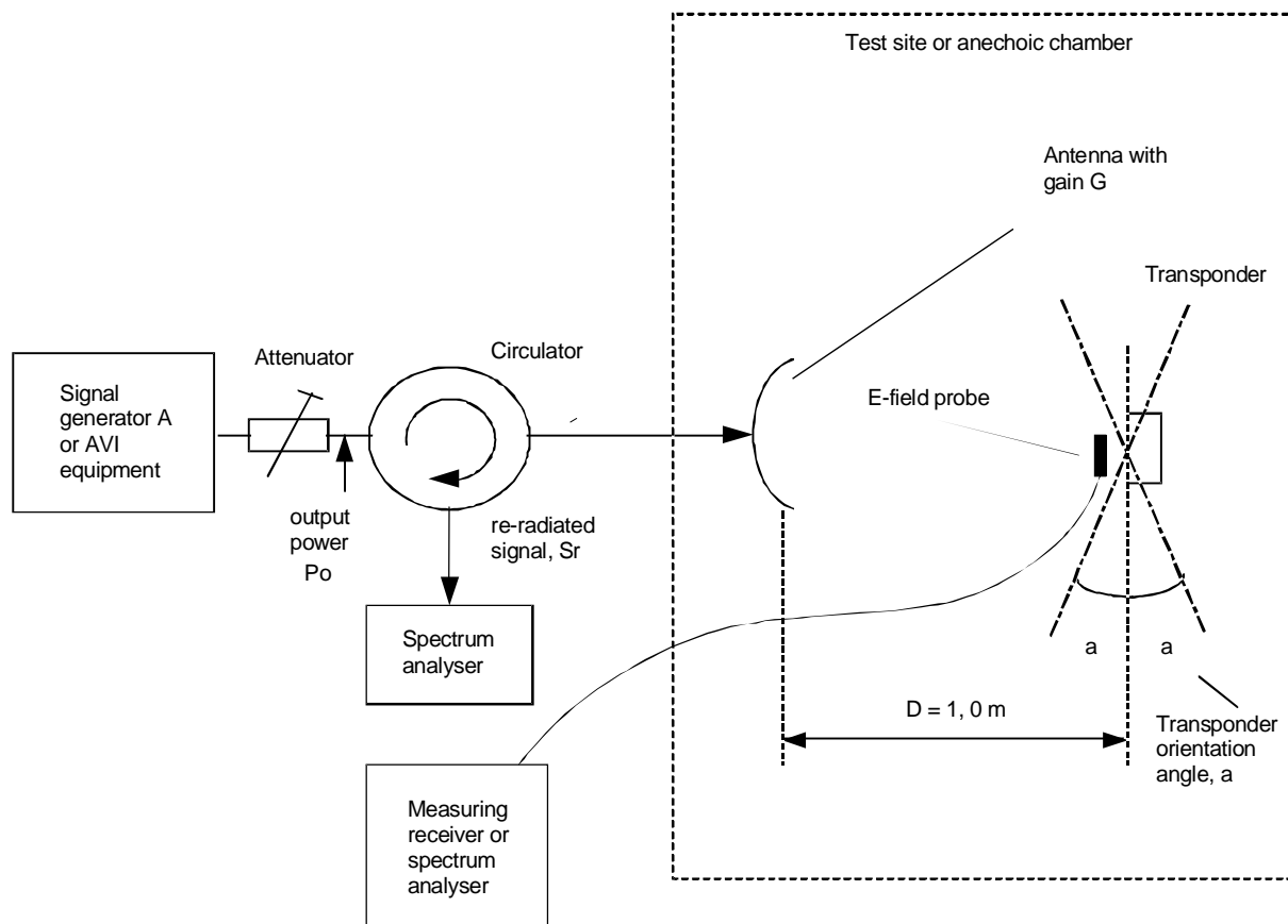
Figure 12: Test arrangement - transponder wake up
