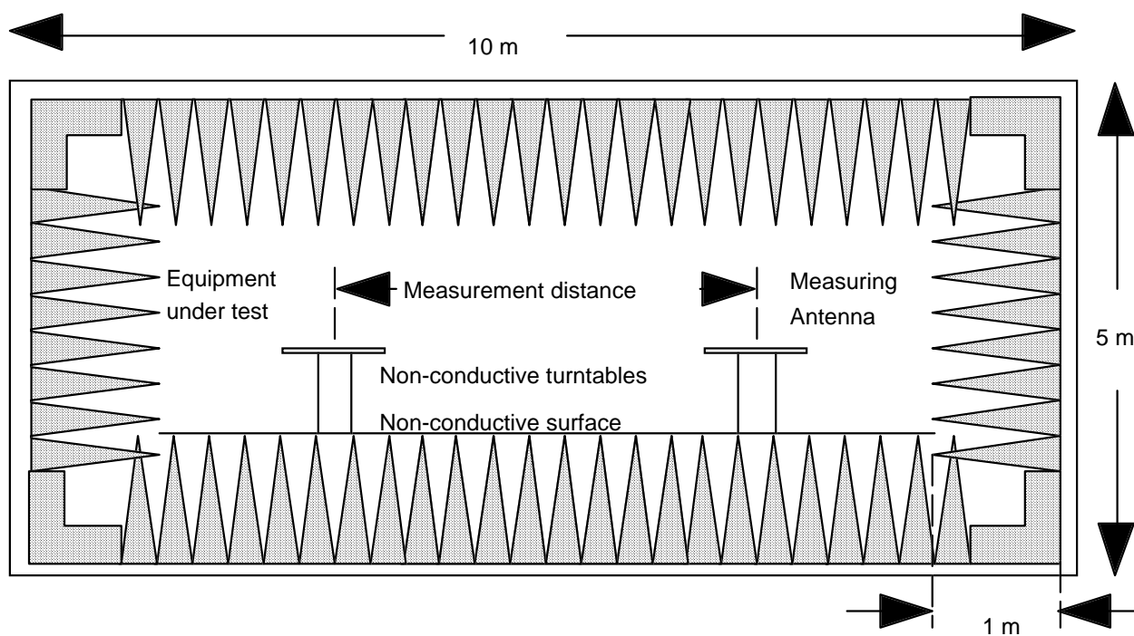
Ground plan
