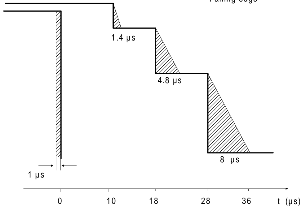
Figure A5.3-1 Time Measurement Uncertainty for the Power Time Mask
