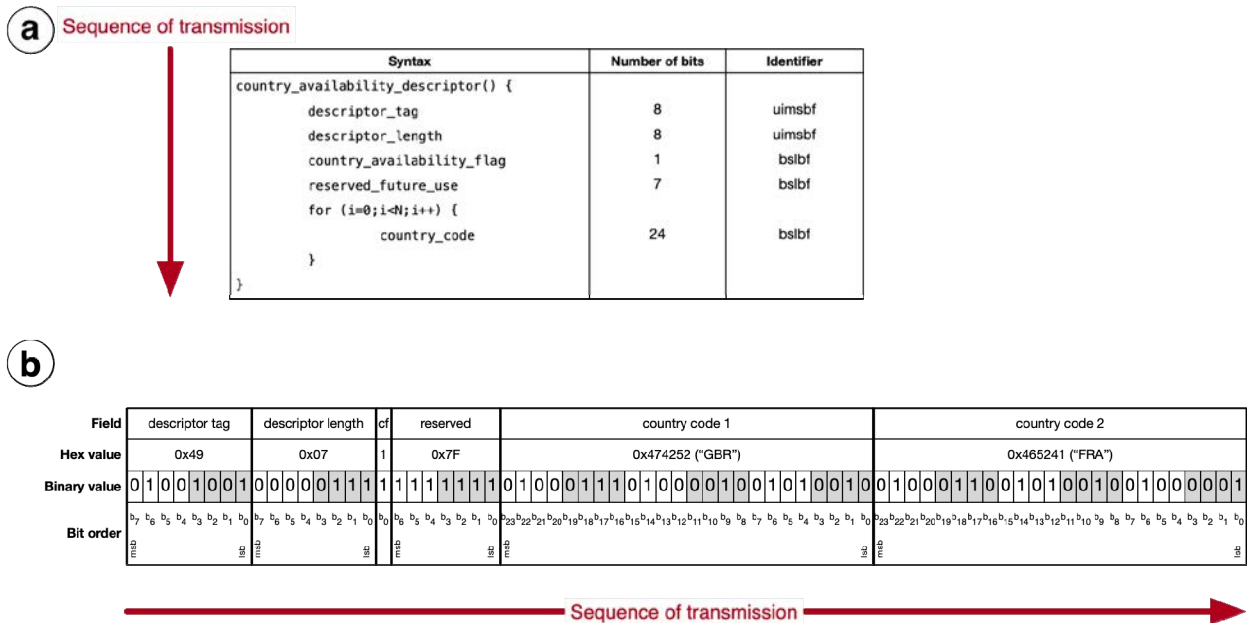
Figure 4: Example of transmission order
