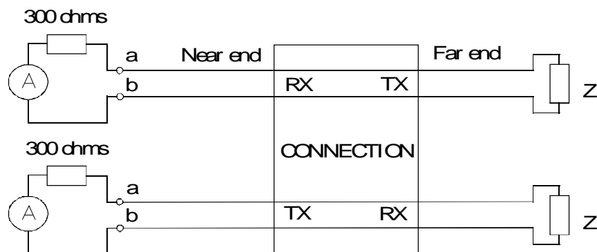
Figure A.7: Power feeding
