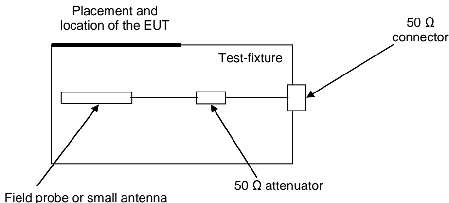
Figure 4: Test fixture
