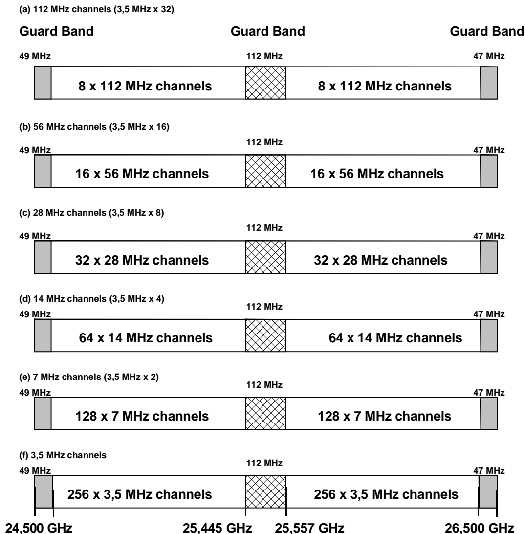
Figure A.1a: Radio frequency channel arrangement
