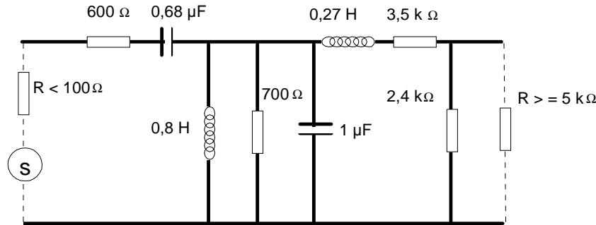
Figure 3: Filter circuit
