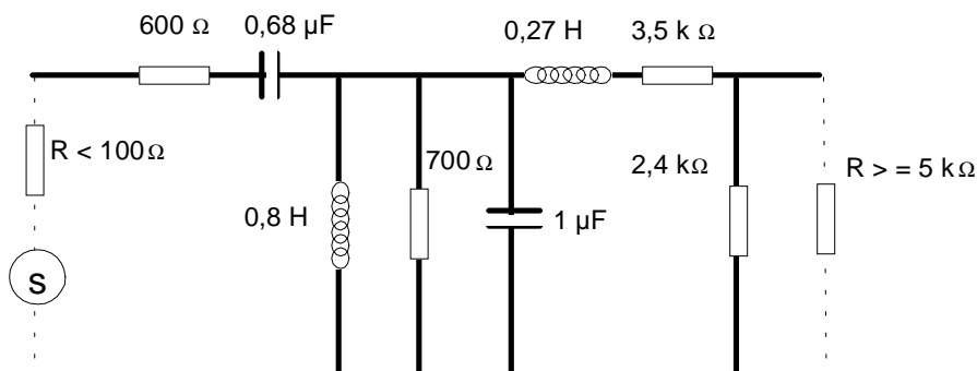
Figure 3: Filter circuit
