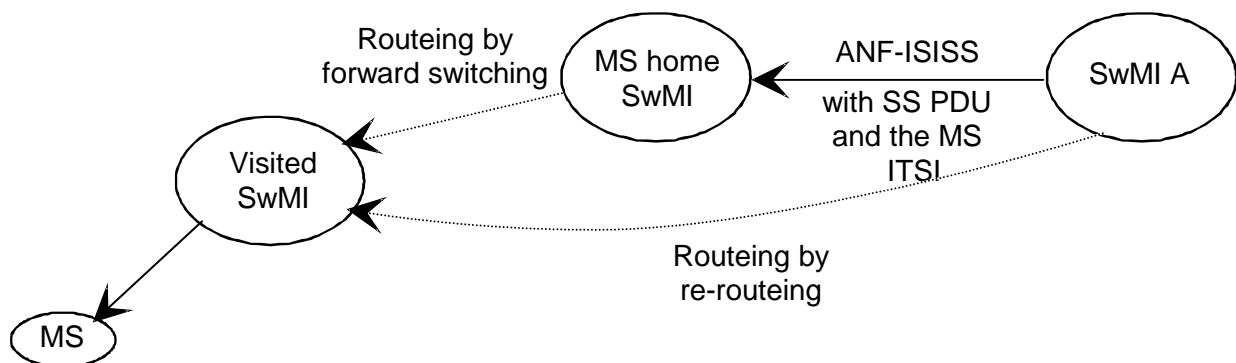
Figure 3: SS PDU addressed individually by an SwMI to an MS
