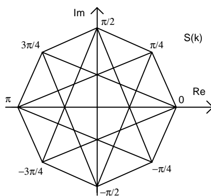
Figure 5.1: \pi/4 -DQPSK modulation symbol constellation and possible transitions
