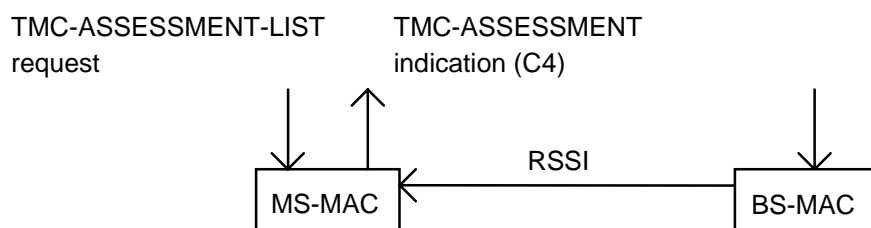
Figure 23.15: Scenario for serving cell channel class assessment
