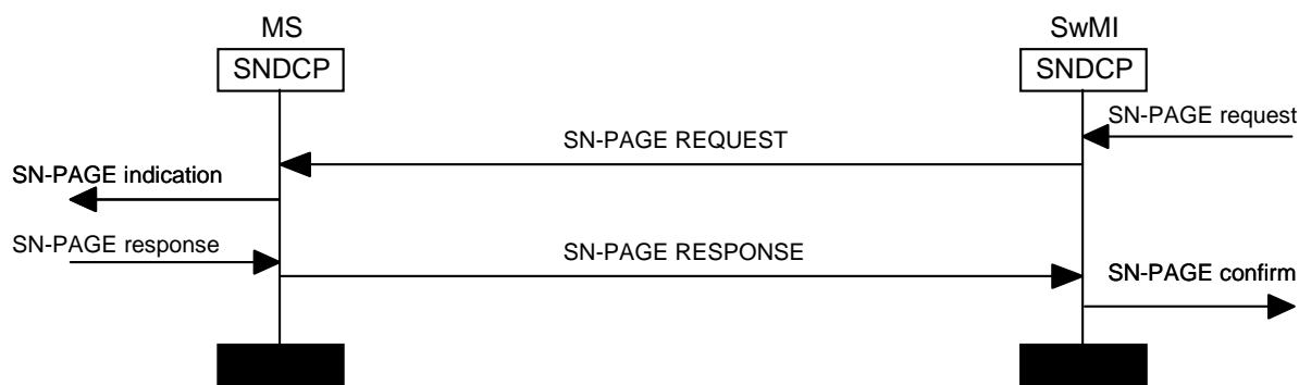
Figure 28.42: SwMI Pages MS, MS SMDCP entity responds
