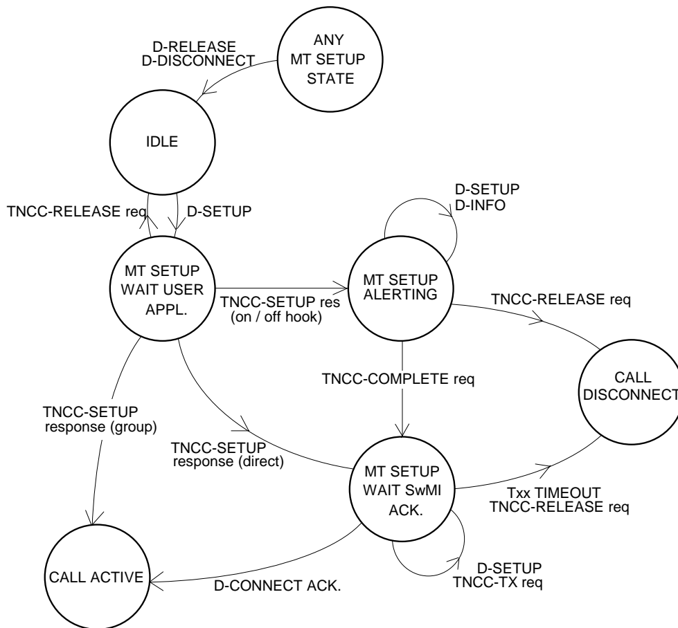
Figure 14.6: Sub state transition diagram for the MT-CALL-SETUP state
