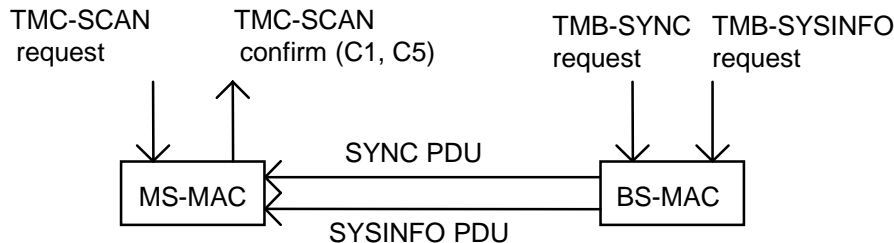
Figure 23.20: Scanning scenario with assessment of channel classes
