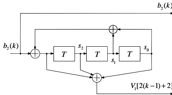
Figure 8.4: RSC encoder
