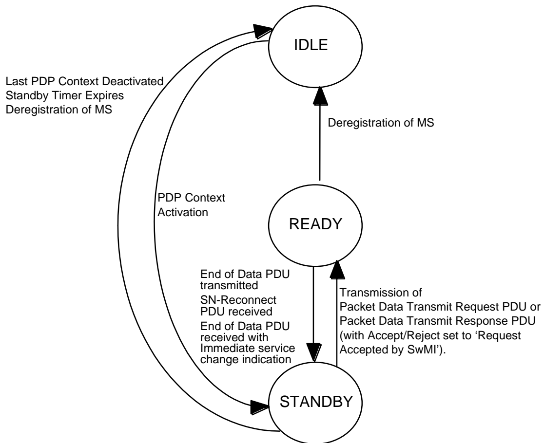
Figure 28.6: Functional SMDCP State Transition Model for SwMI
