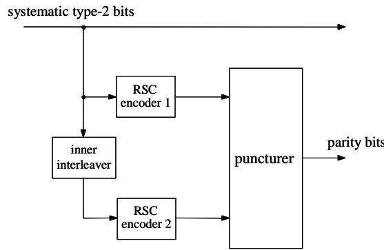
Figure 8.3: PCCC encoder
