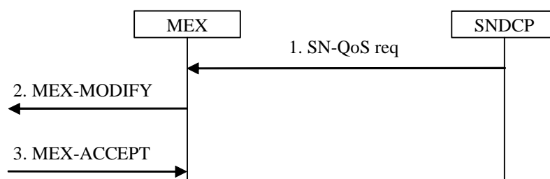
Figure 30.10: QoS modification procedure – SNDSCP originated
