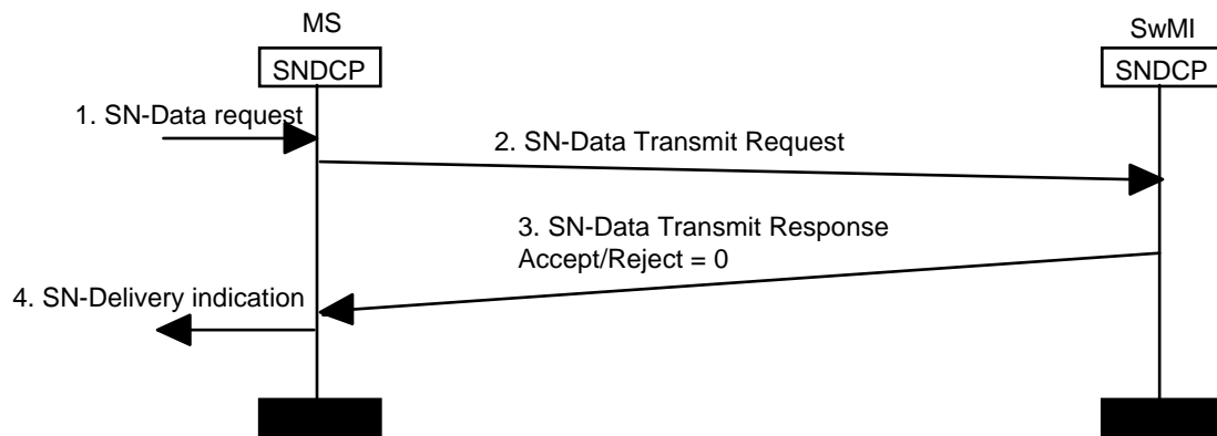
Figure 28.36: Acknowledged service, SwMI rejects request
