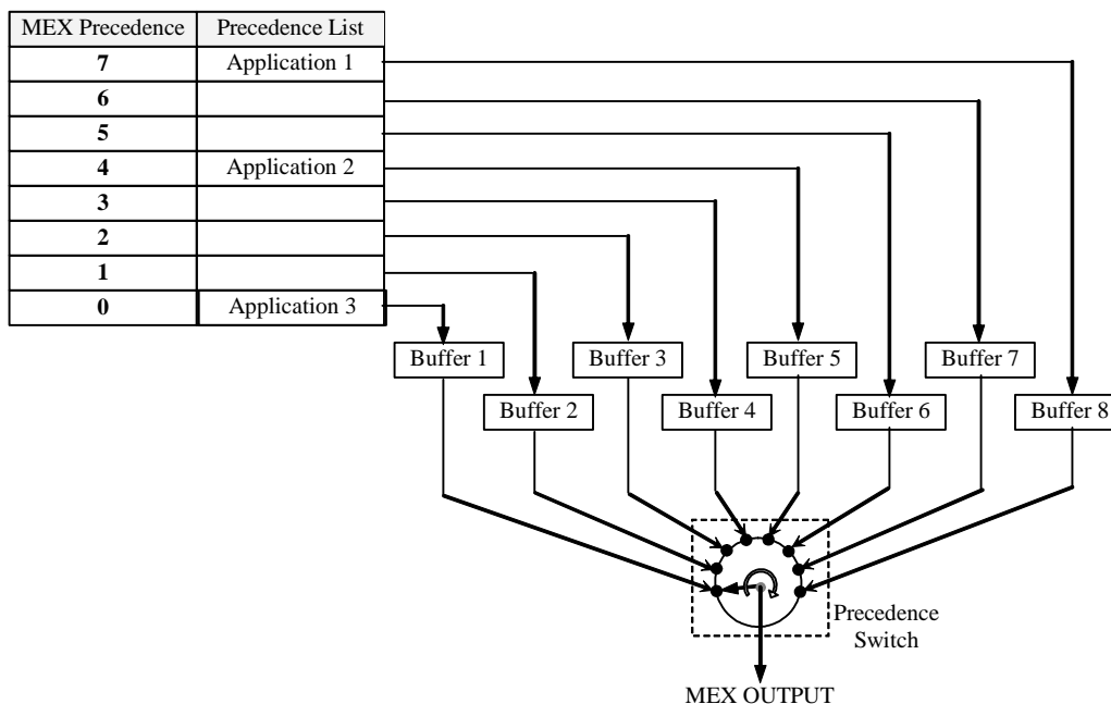
Figure 30.4: MEX Precedence
