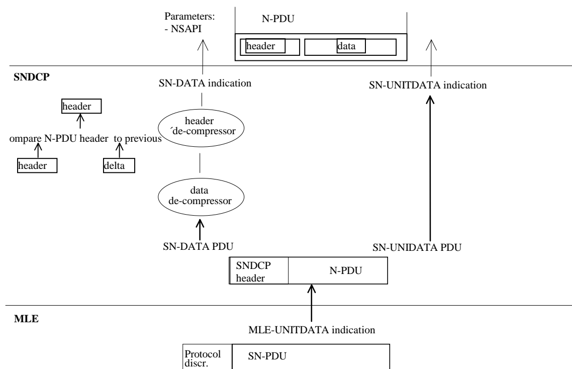
Figure 28.8: SDCP model for receiver end
