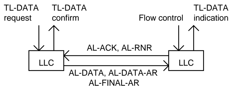
Figure 22.32: Flow control PDU exchange
