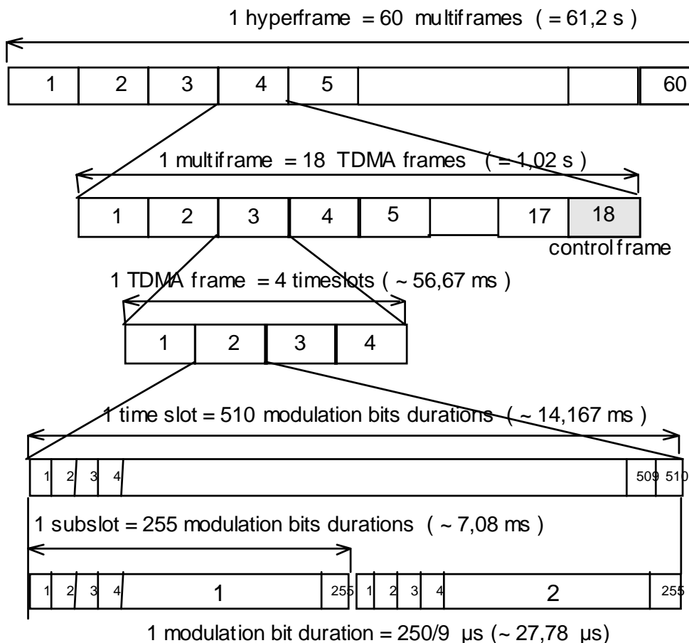
Figure 9.1: TDMA structure
