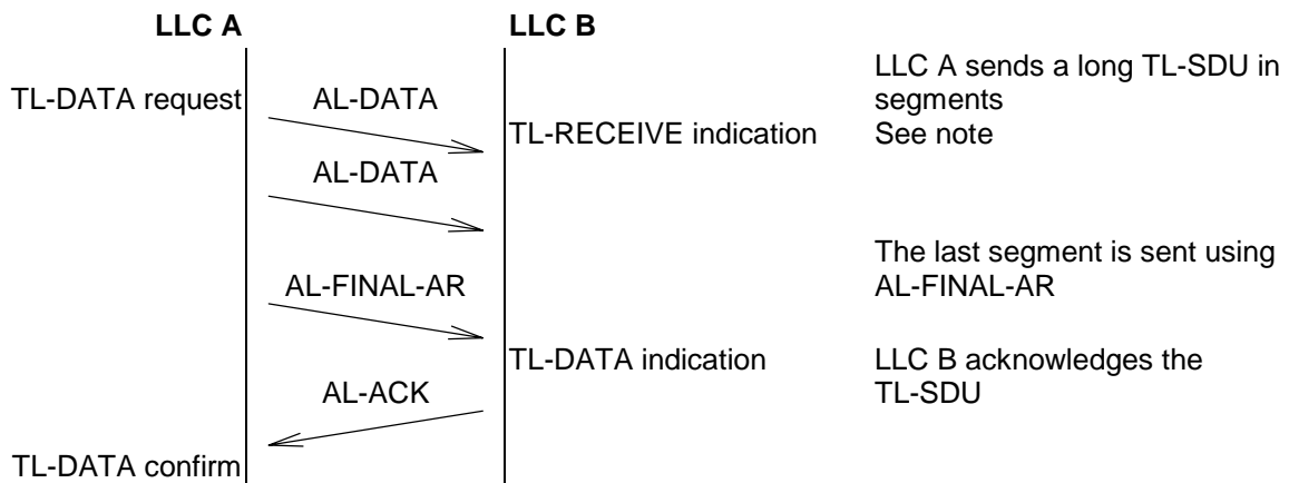
Figure 22.22: PDU exchange in a unidirectional transfer
