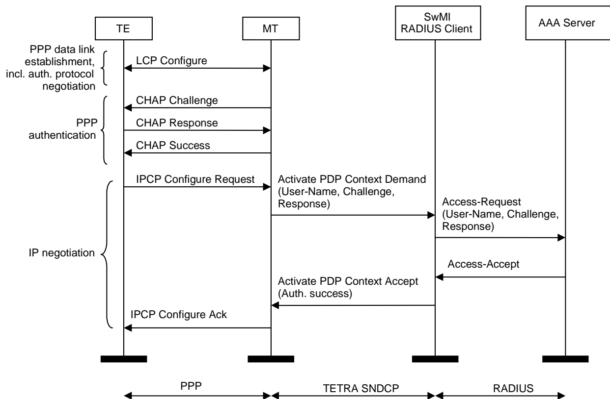
Figure 28.38: A successful authentication with CHAP
