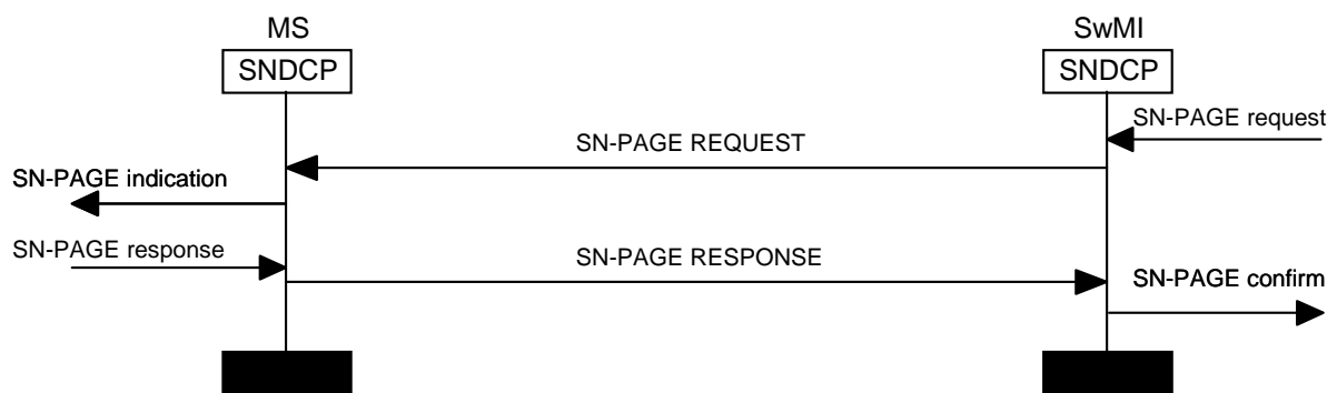
Figure 28.36: SwMI Pages MS, MS SMDCP entity responds
