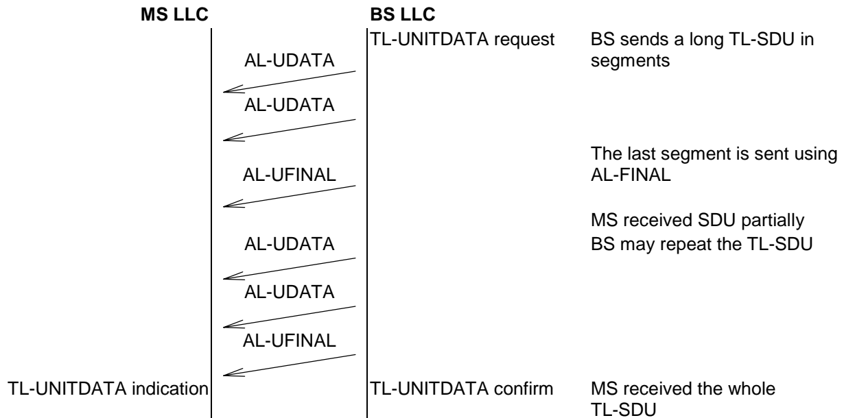
Figure 22.28: PDU sending in a unidirectional transfer
