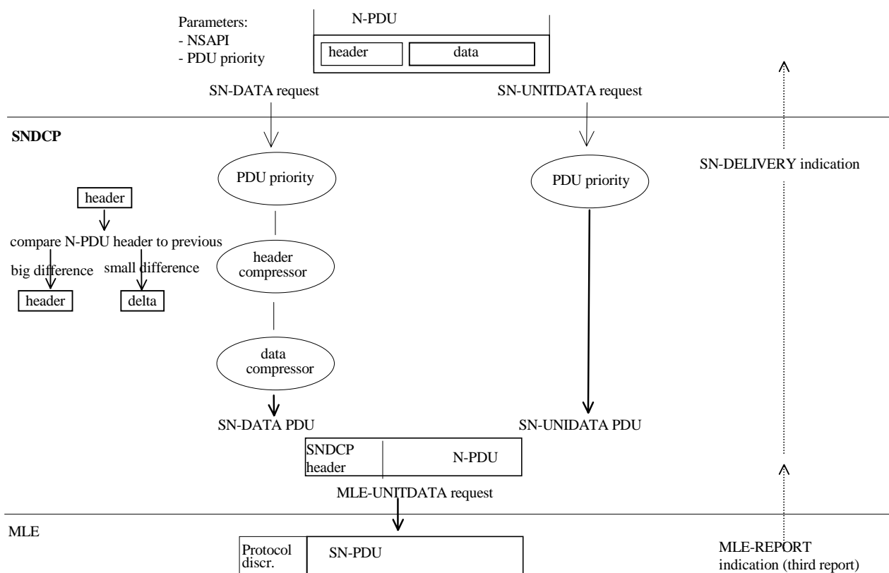
Figure 28.7: SDCP model for transmitting end
