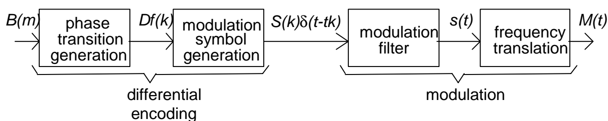
Figure 4: Block diagram of the modulation process
