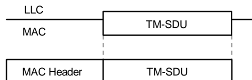
Figure 95: General format of the MAC PDU
