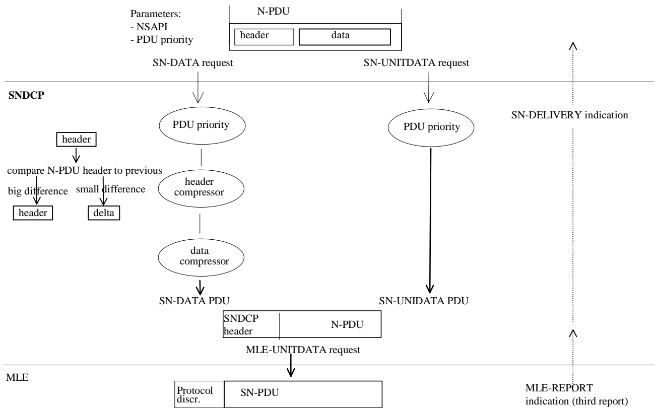
Figure 186: SNDP model for transmitting end
