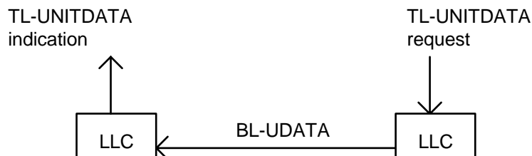
Figure 109: PDU exchange in unacknowledged mode
