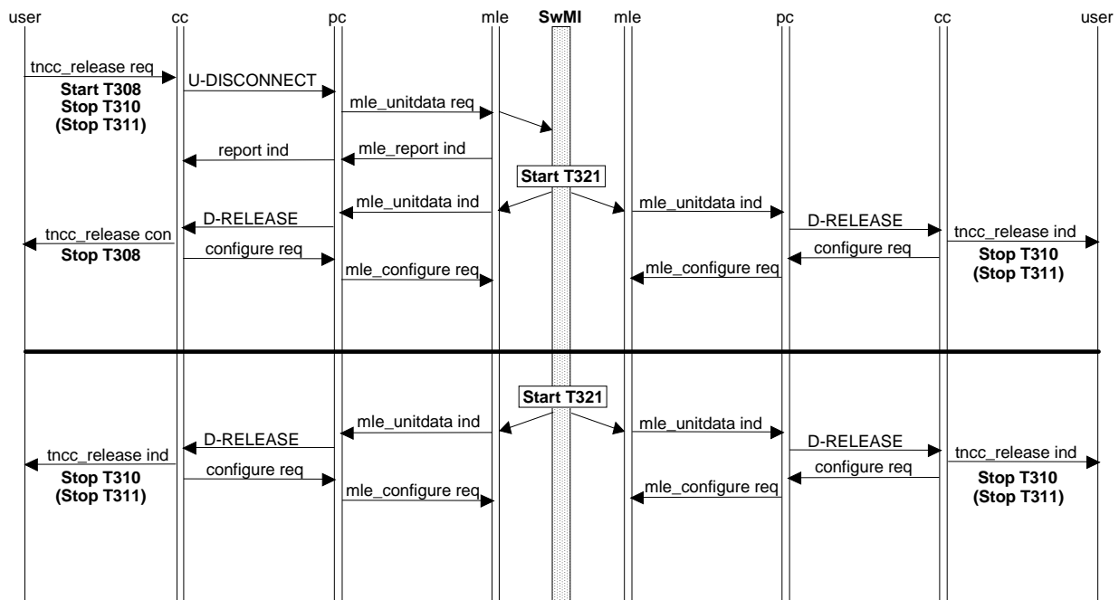
Figure 38: Group call - request-to-disconnect
