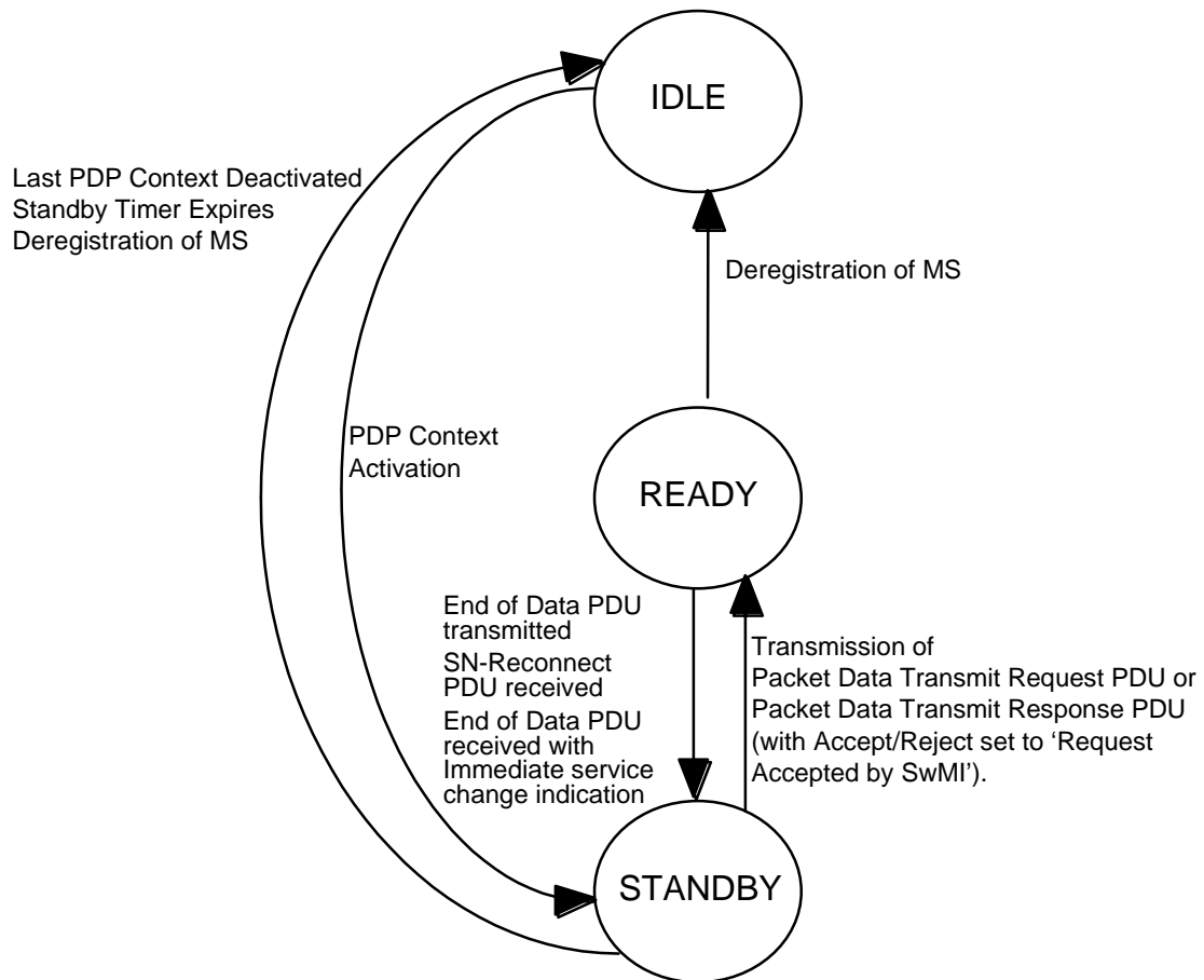
Figure 185: Functional SNDCP State Transition Model for SwMI
