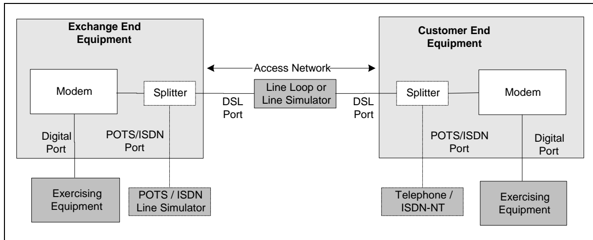
Figure 3: DSL Access System Configuration
