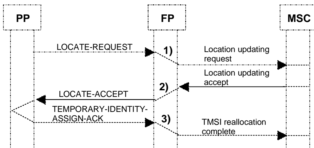
Figure 18: Location registration
