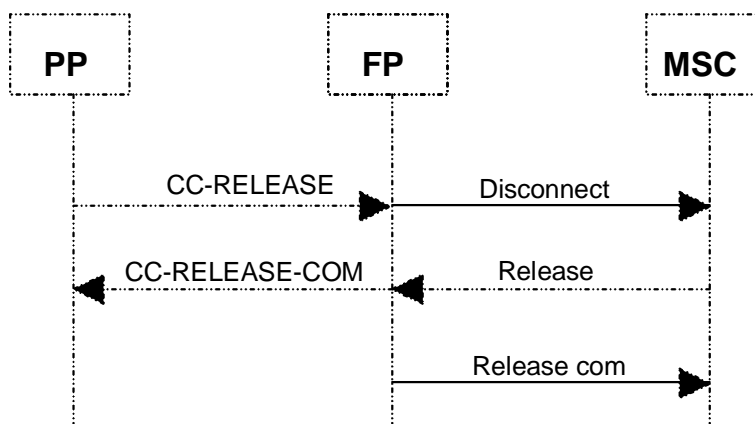
Figure 8: Normal release initiated by the PP
