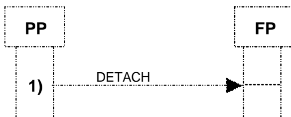
Figure 40: Detach procedure
