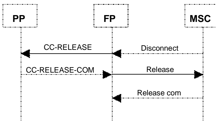
Figure 10: Normal MSC initiated call release with no tones
