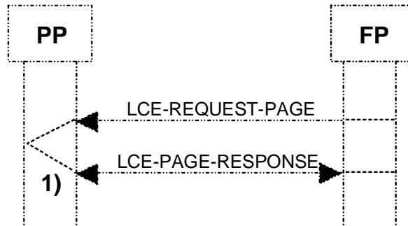
Figure 43: Paging procedure
