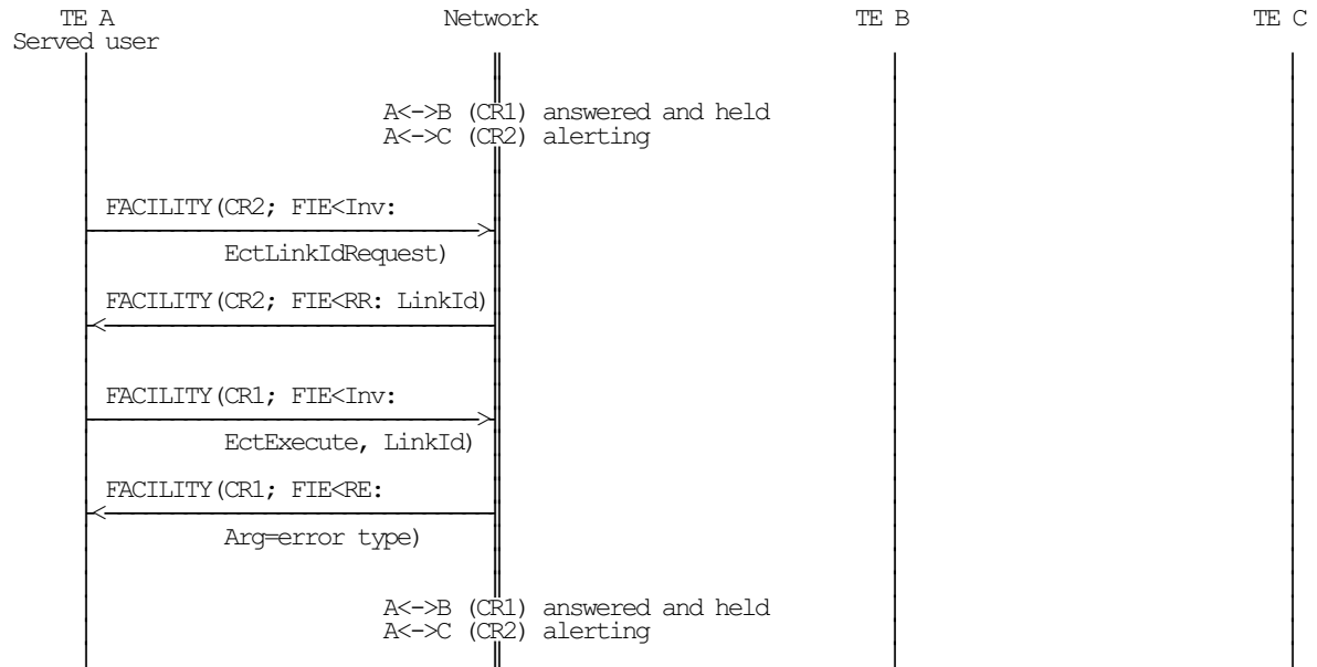
Figure A.4: ECT explicit invocation - EctExecute fails
