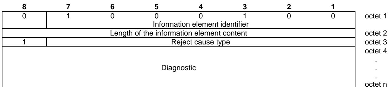
Figure 22: Reject Cause information element
