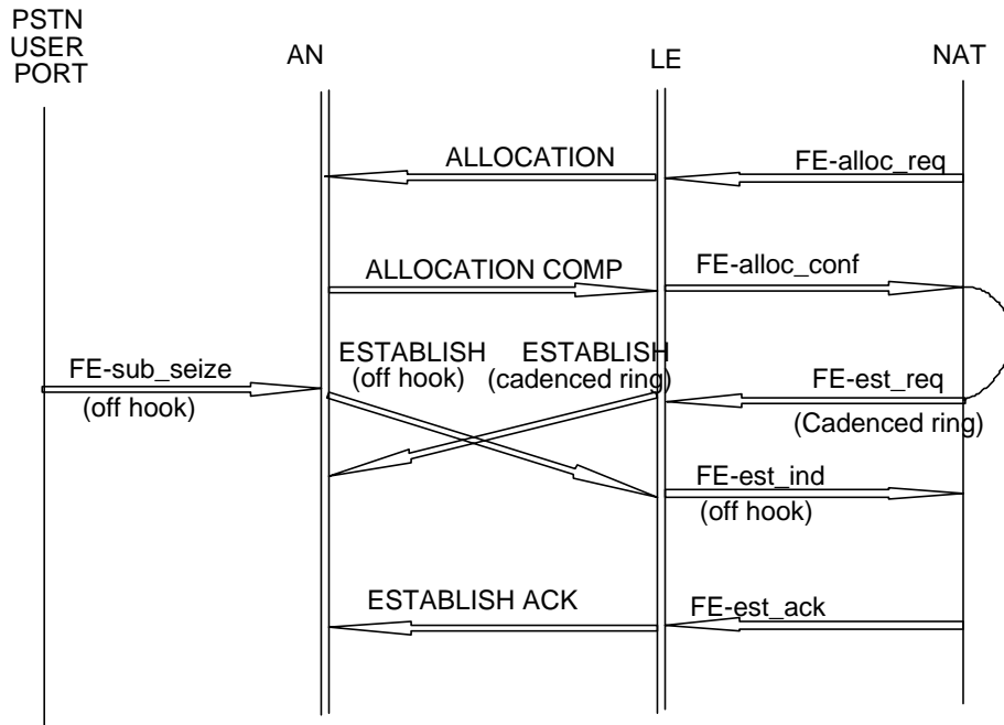
Figure E.13: PSTN call collision, originating call has priority
