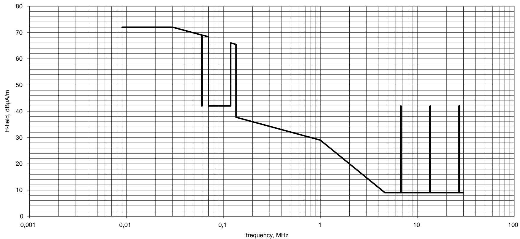
Figure B.1: Radiated H-field at 10 m distance
