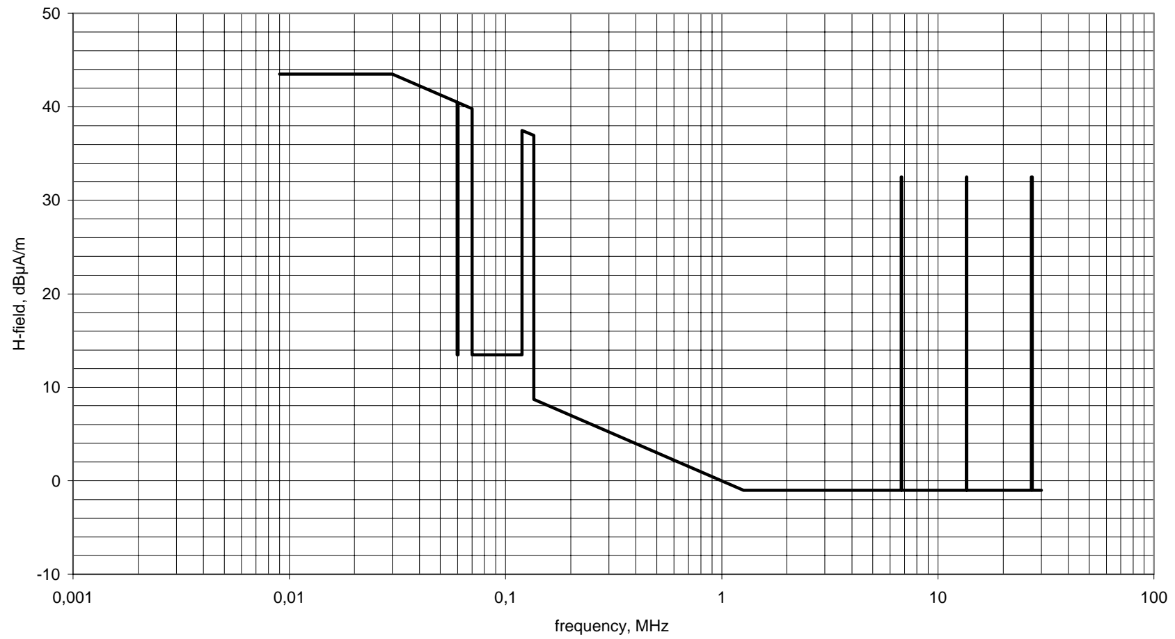
Figure J.1: Radiated H-field at 30 m distance
