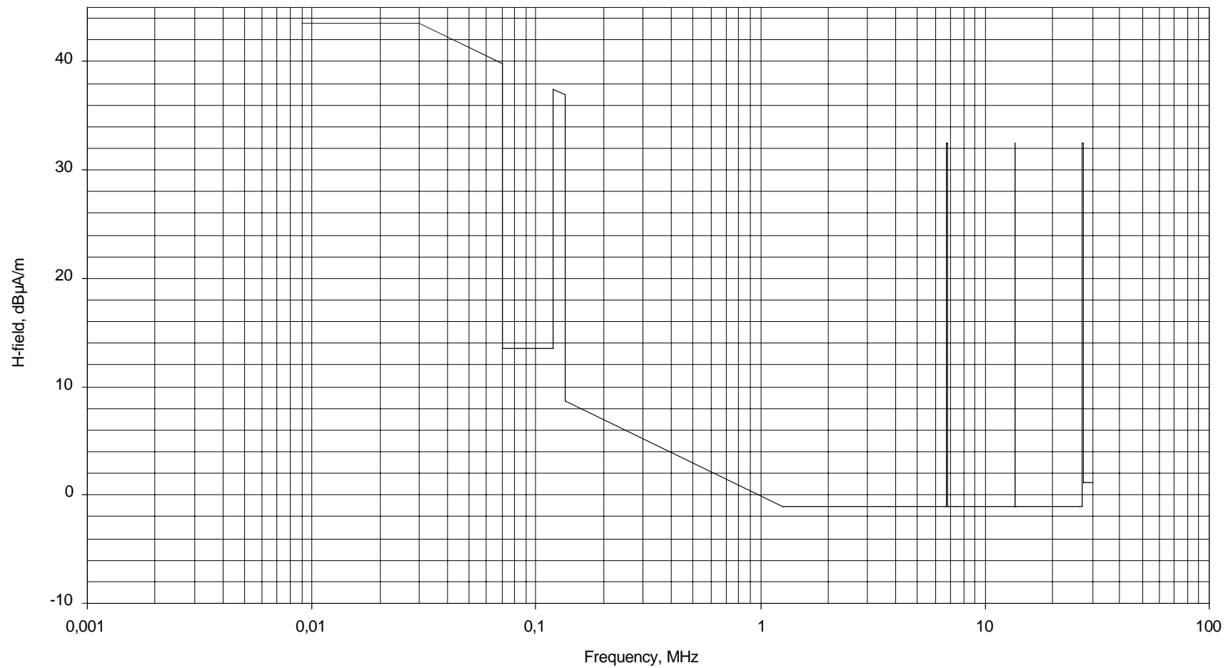
Figure K.1: Radiated H-field at 30 m distance
