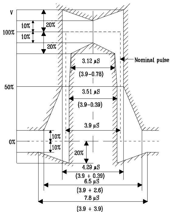
Figure 2: Pulse mask for single pulse
