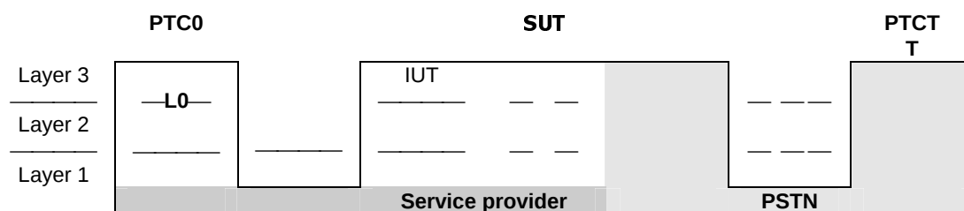
Figure 3: Combination of the remote and multi-party test methods with interworking with PSTN
