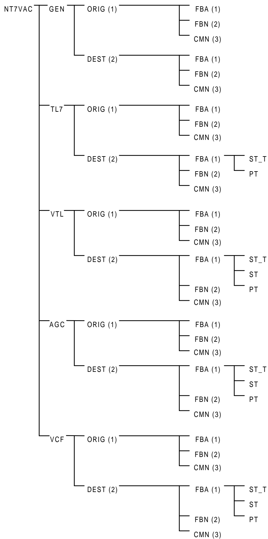
Figure 1: Test suite structure
