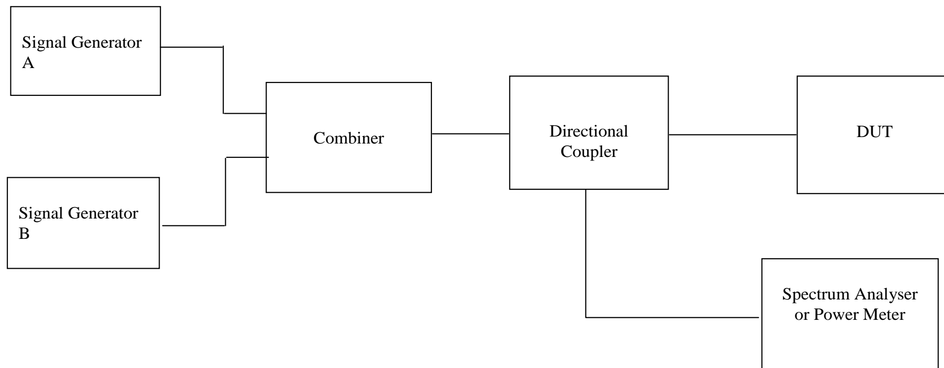
Figure 11: Measurement arrangement
