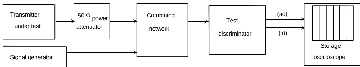
Figure 10: Measurement arrangement
