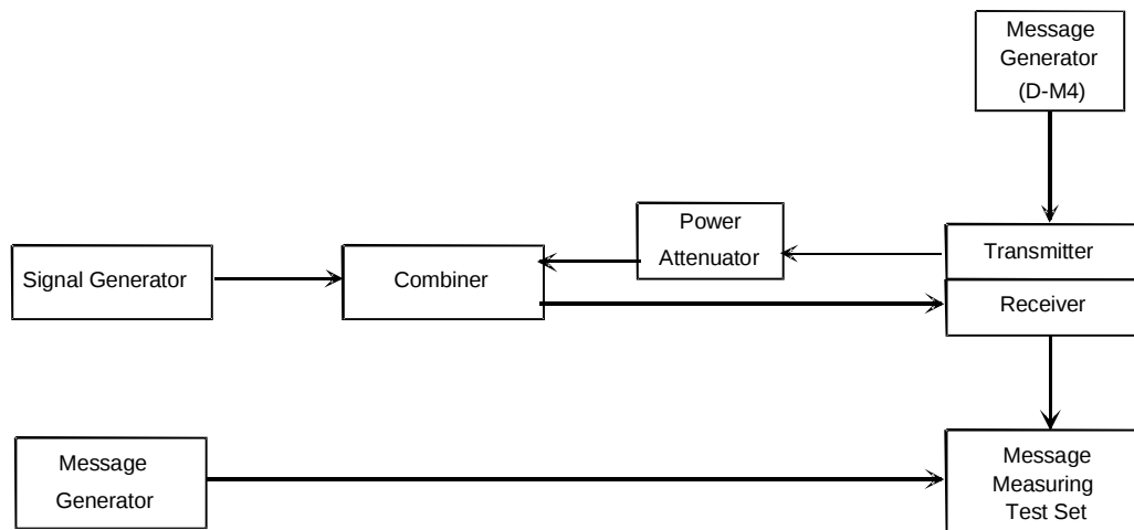
Figure 22: Measurement Arrangement
