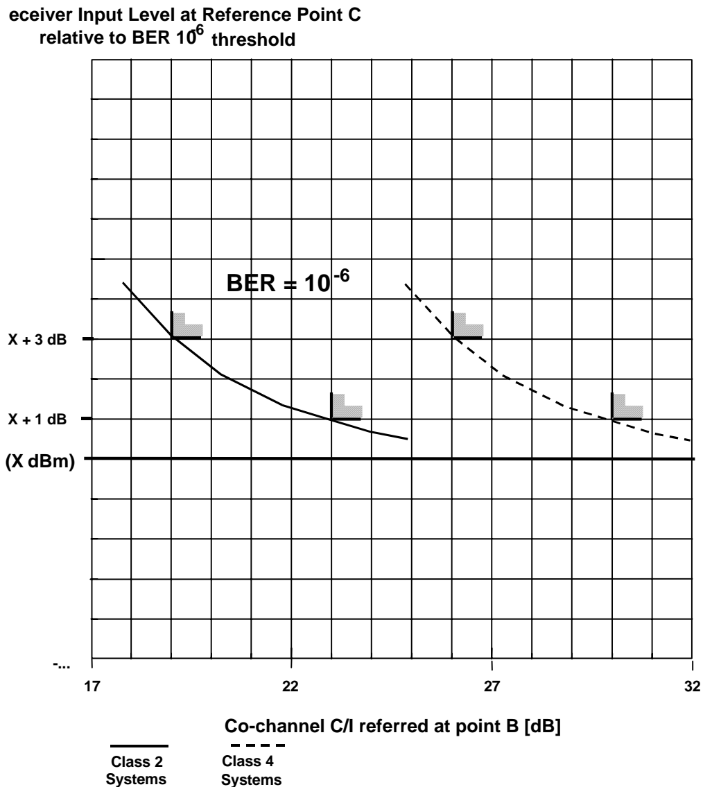
Figure A.2: Co-channel interference threshold degradation
