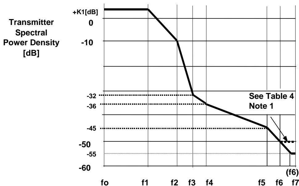
Figure 3c: Limits of spectral power density for Class 5a systems
