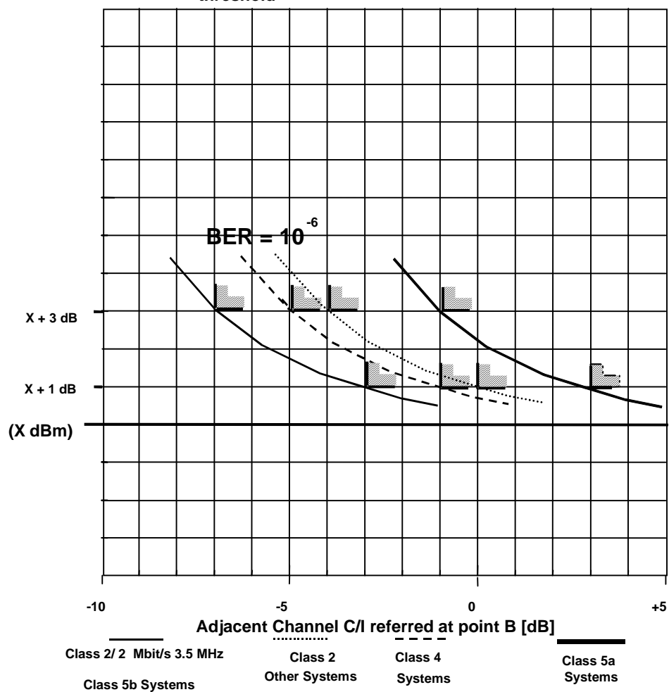
Figure A.4: First adjacent channel interference threshold degradation
