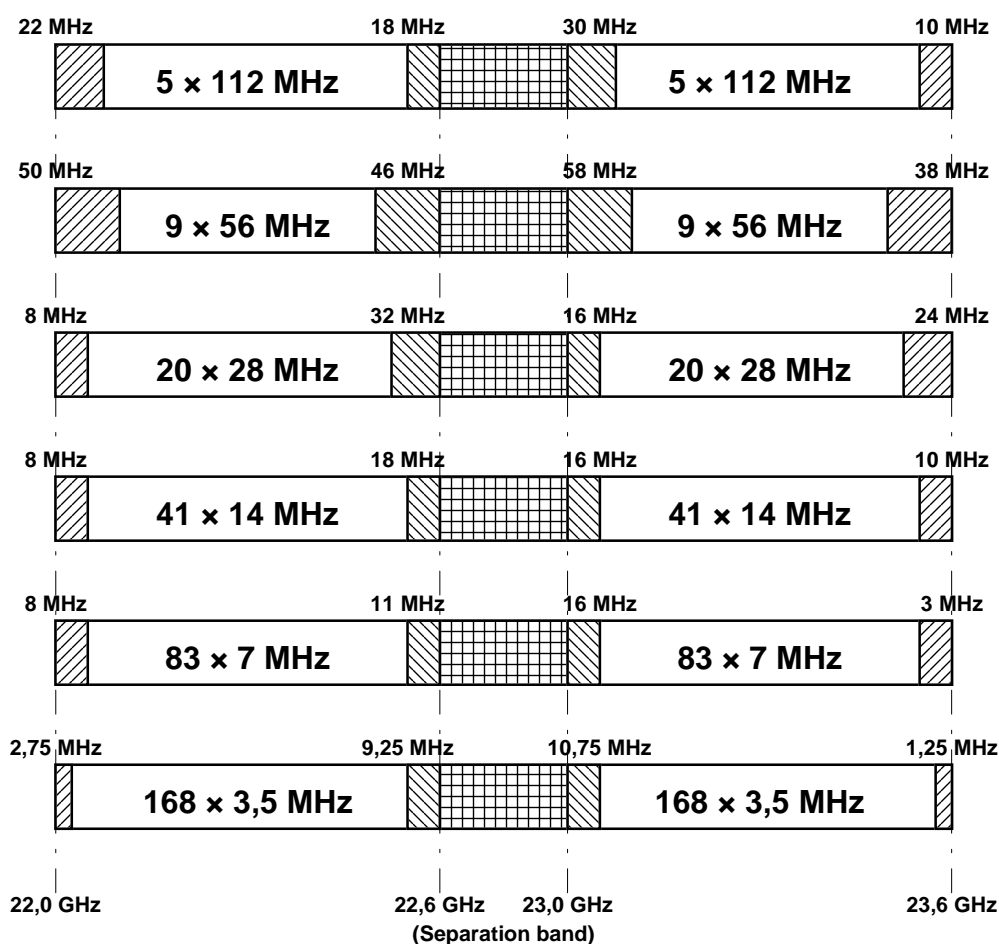
Figure A.1: Radio frequency channel arrangement
