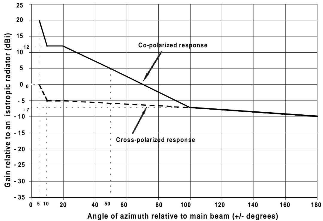
Figure A.2 a): Type A antenna radiation pattern (under test conditions)
